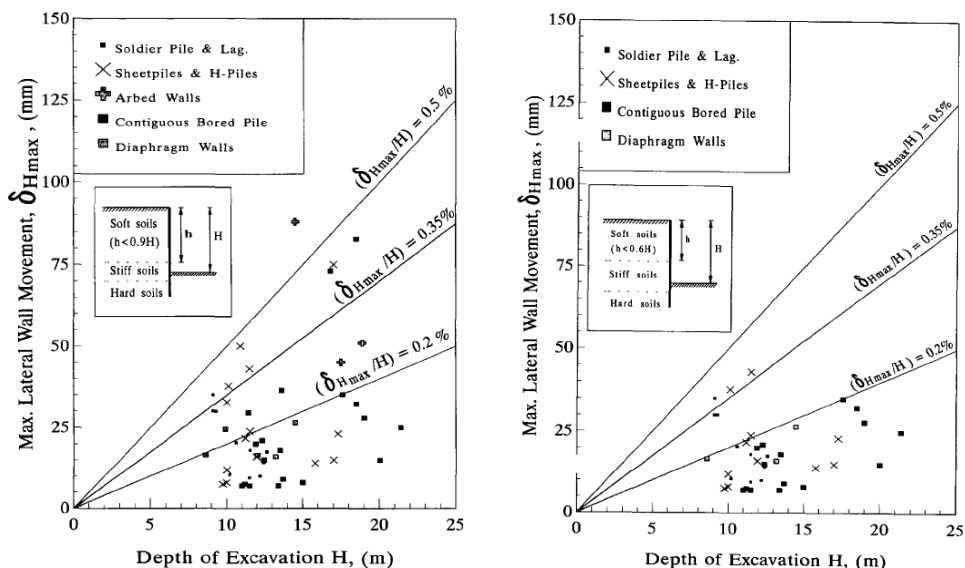
Figure 2.8 Observed Maximum Lateral Wall Deflection for Excavation by Five Types of Walls (left, h < 0.9H and right, h < 0.6H ) in the Construction of CTE
