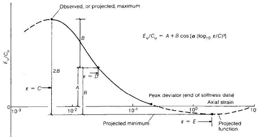
Figure 2.24 Curve and Equation Fitting to Stiffness-Strain Data (Jardine et.al, 1986)
