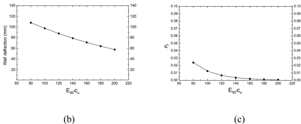
Figure 5.10 Effect of E_{50}/c_u on (a) Sensitivity Parameter (b) Wall Deflection (c) P_f
