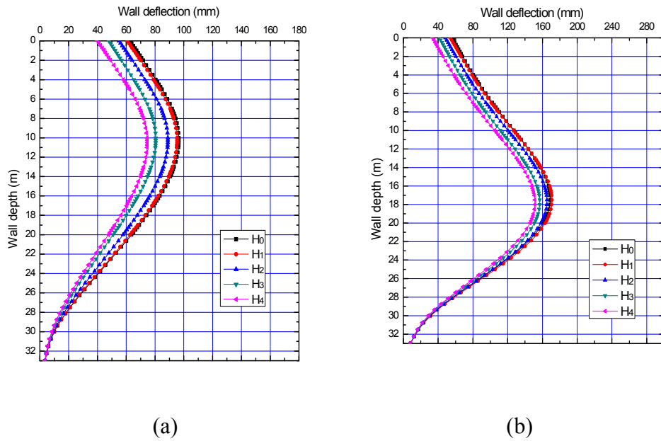
Figure 3.24 Wall Deflection at Excavation Depth (a) h = 8\text{m} (b) H_e = 20\text{m}
