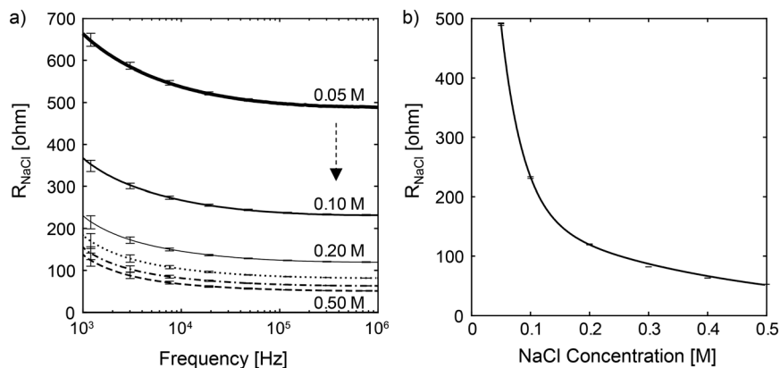
Fig. 3 (a) Plot of the mean electric resistance, R_{NaCl} , as a function of frequency for NaCl solutions at molar concentrations of 0.05 M, 0.10 M, 0.20 M, 0.30 M, 0.40 M and 0.50 M, respectively. The vertical bars denote the upper and lower bounds of measurements at selected frequencies. (b) Plot of R_{NaCl} as a function of NaCl molar concentration at f = 724 kHz. The vertical bars represent the upper and lower bounds of measurements at different NaCl concentrations. The solid line is the curve fitting line. By knowing the electric resistance of urine, R_{urine} , we can determine the conductive ion concentration, [C]_{urine} , through interpolation.
