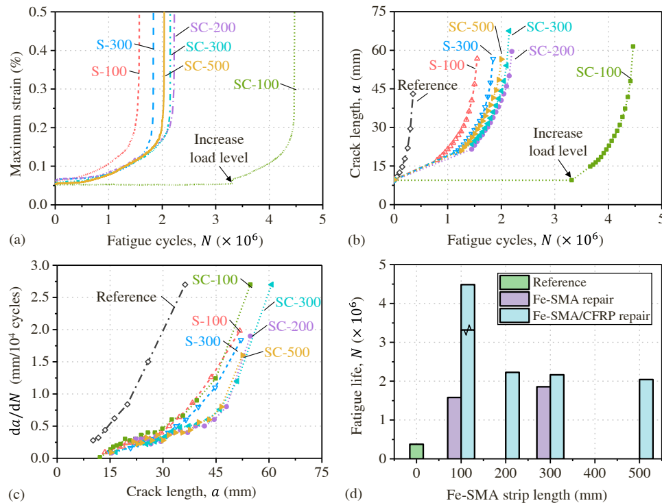
Fig. 10. Fatigue behavior. (a) Evolution of the maximum strain reading of SG5 on Fe-SMA strip or CFRP sheet. (b) Fatigue crack growth behavior. (c) Crack growth rate. (d) Fatigue lives of all specimens.
