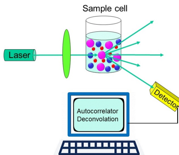
Figure 8. A simplified schematic illustration of DLS.
