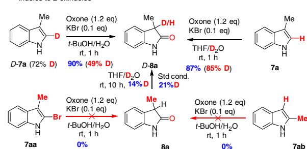
Fig. 5 Oxone-Halide oxidation of indoles to 2-oxindoles. a Substrate scope for oxone-KBr oxidation of C3-substituted indoles to 2-oxindoles. b Total syntheses of (±)-desoxyseroline, (±)-physovenol methyl ether and (±)-esermethole. c Controlled experiments for possible mechanism for the oxone-KBr oxidation of C3 substituted indoles to 2-oxindoles. TBAHS Tetrabutylammonium hydrogen sulfate
