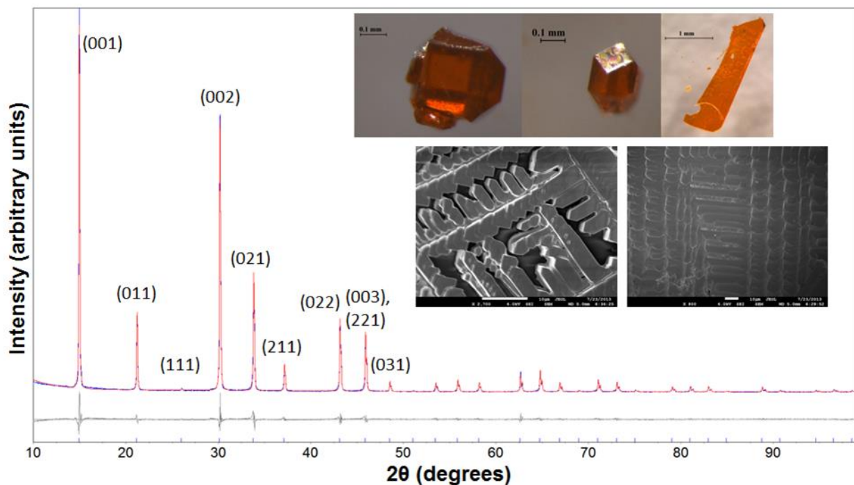
Figure 1. Powder X-ray diffraction pattern of \text{MAPbBr}_3 , which has been indexed assuming cubic symmetry ( Pm\bar{3}m ). Data were collected from a finely ground powdered sample prepared from the solution growth method first described by Poglitsch et al. 7 Inset – elongated dodecahedral single crystals and scanning electron microscopy image of \text{MAPbBr}_3 that were drop-casted onto a glass substrate from a solution of \text{CH}_3\text{NH}_2 and lead acetate in \text{HBr} , which was subsequently heated at 100^\circ\text{C} for 2-3 mins to dry the sample.
