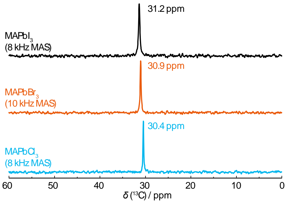
Figure 8. ^{13}\text{C} solid-state MAS NMR spectra at room temperature using a direct acquisition with proton decoupling. The ^{13}\text{C} spectra for the I, Br and Cl appear at 31.2, 30.9 and 30.4ppm respectively
