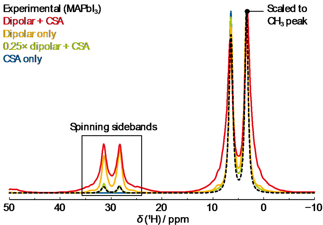
Figure 7. Experimental and simulated ^1\text{H} solid-state MAS NMR spectra.
