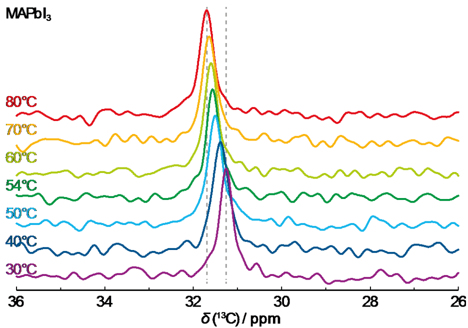
Figure 9. ^{13}\text{C} solid-state MAS NMR spectra of \text{CH}_3\text{NH}_3\text{PbI}_3 at temperatures between 30°C to 80°C.
