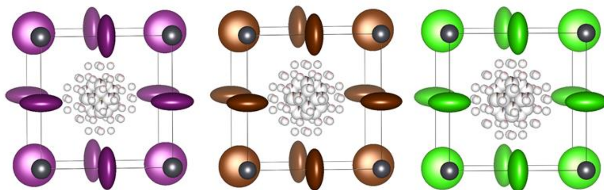
Figure 13. Refined structures of the \text{MAPbI}_3 (left), \text{MAPbBr}_3 (centre) and \text{MAPbCl}_3 (right) indicating the disordered arrangement of the MA groups and the highly anisotropic displacement ellipsoids of the halogen ions (shown with a 90% probability).
