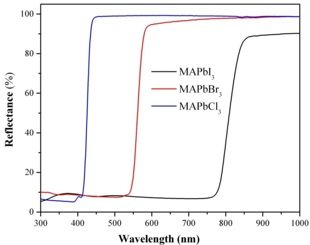
Figure 3. Diffuse reflectance spectra for \text{MAPbX}_3
