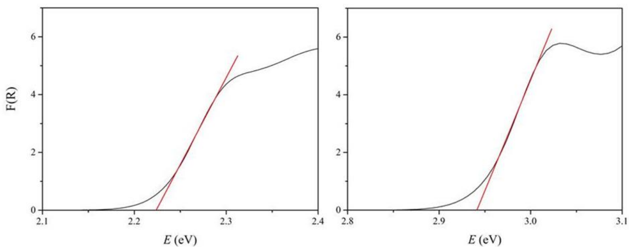
Figure 4. Kubelka-Munk spectra for the \text{MAPbBr}_3 (left) and \text{MAPbCl}_3 (right) revealing optical band-gaps of 2.22 and 2.94 eV respectively.
