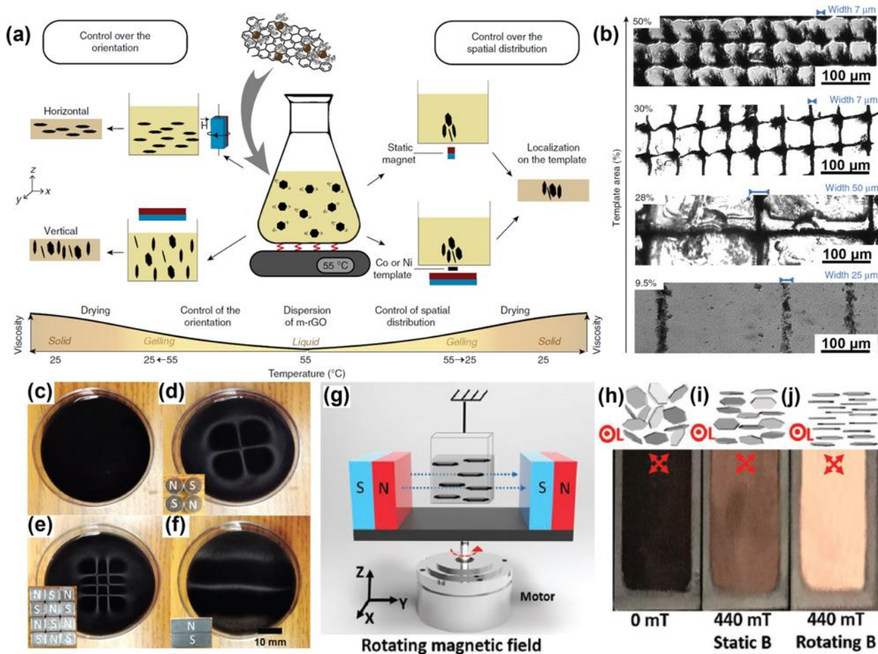
Fig. 15 Controlled orientation of 2D nanomaterials assisted by magnetic field. (a) Schematic illustration of magnetic control over orientation or spatial distribution of magnetized reduced graphene oxide (m-rGO) flakes. (b) Optical micrographs of patterned poly(2-acrylamido-2-methyl-1-propanesulfonic acid) (PAMPS) composites with 0.065 vol% magnetically responsive rGO flakes of decreasing template area and various line width. Reproduced from ref. 60 with permission from Springer Nature. Photographs of 0.1 wt% graphene suspension with (c) no magnet field and (d)–(f) magnets of different shapes and configurations placed underneath for magnetic field sensing and display. Reproduced from ref. 222 with permission from John Wiley and Sons. (g) Schematic of experimental setup to generate a rotating magnetic field for planar alignment of graphene sheets. (h)–(j) Schematic representation and snapshots of white light birefringence/transmission images of graphene suspension with different magnetic field conditions: (h) without magnetic field, (i) under static magnetic field in x-y direction, and (j) under rotating magnetic field in the x-y plane. The symbol L represents the incident white light in x direction. Reproduced from ref. 221 with permission from John Wiley and Sons.
