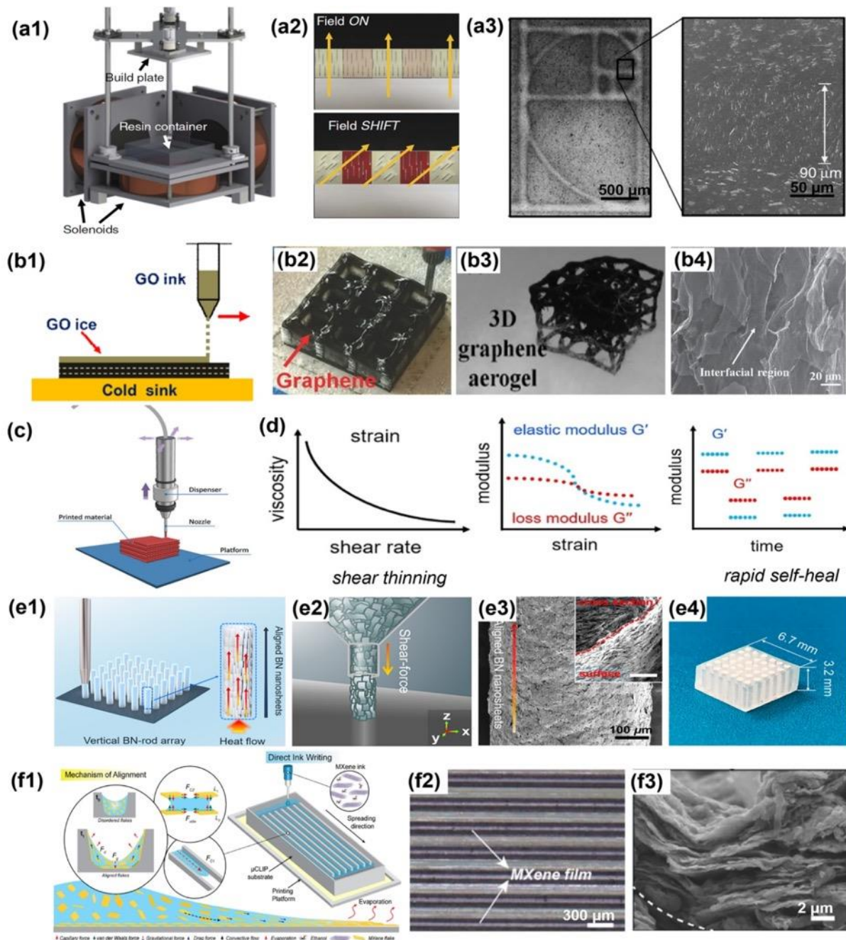
Fig. 20 Representative 3D printing techniques combined with 2D materials alignment. (a1) Schematic representation of the 3D magnetic-printer setup. (a2) The 3D magnetic printing process with programmable magnetic field shift and selective polymerization. (a3) The printed micro-architectures showing complex particle orientation. Reproduced from ref. 281 with permission from Springer Nature. (b1) Schematic of freeze casting assisted 3D printing of graphene aerogel. (b2) 3D printing of graphene suspension. (b3) Thermally reduced 3D ultralight graphene aerogel. (b4) Cross-sectional SEM image showing interfacial region along deposition direction. Reproduced from ref. 282 with permission from John Wiley and Sons. (c) Schematic diagram of direct ink writing (DIW). Reproduced from ref. 298 with permission from Royal Society of Chemistry. (d) Favored rheological properties of typical DIW ink with shear thinning and rapid self-healing properties. Reproduced from ref. 287 with permission from John Wiley and Sons. (e1) Schematic illustration of the 3D vertical printing of a BN array through DIW method. (e2) Schematic illustration of BNNSs alignment by shear force from the fine nozzle during extrusion. (e3) Morphology of the printed BN rod showing vertically aligned BNNSs. (e4) Scalable BN array encapsulated into a PDMS matrix. Reprinted with permission from ref. 294. Copyright (2019) American Chemical Society. (f1) Schematic of the \text{Ti}_3\text{C}_2\text{T}_x MXene alignment by capillarity-driven DIW v via microcontinuous liquid interface production ( \mu\text{CLIP} ). (f2) Representative top view of deposited MXene films on patterned substrates. (f3) Printed MXene films showing alignment. Reprinted with permission from ref. 295. Copyright (2021) American Chemical Society.
