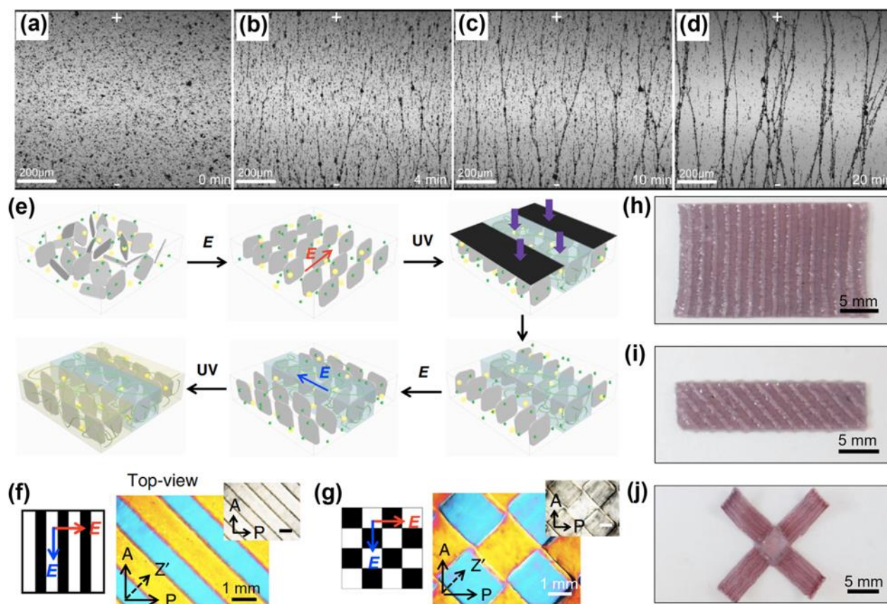
Fig. 16 Controlled orientation induced by electric field. (a)-(d) Optical micrograph images of graphene nanoplatelets alignment in liquid epoxy resin by AC electric field ( E ) as a function of time (0 to 20 min). (a) Random orientation of graphene nanoplatelets before applying electric field, and after applying electric field for (b) 4 min, (c) 10 min and (d) 20 min. Reproduced from ref. 233 with permission from Elsevier. (e) Schematic representation of patterned anisotropic hydrogel by multi-step electrical orientation and photolithographic polymerization with different electric field ( E ) directions and use of ultraviolet (UV) light. (f) and (g) Polarizing optical microscope (POM) images showing hydrogel patterns with different nanosheet alignment. A: analyzer, P: polarizer, Z': axis of the tint plate. (h)-(j) Photos of the patterned anisotropic hydrogels. Reproduced from ref. 232 with permission from Springer Nature.
