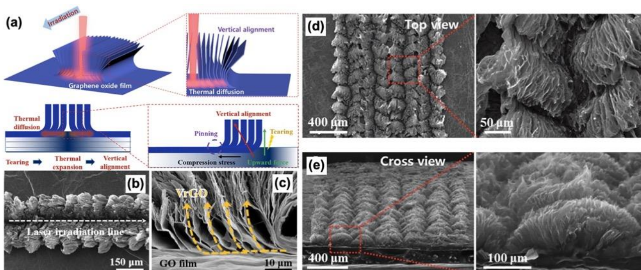
Fig. 11 Vertical alignment of reduced graphene oxide nanosheets by laser irradiation. (a) Schematic of the CO 2 laser irradiation fabrication process of vertically aligned nanostructure. (b) and (d): Top view of the vertically aligned nanosheets. (c) and (e): Cross-sectional view of the as-fabricated nanostructure. Reproduced from ref. 186 with permission from Elsevier.
