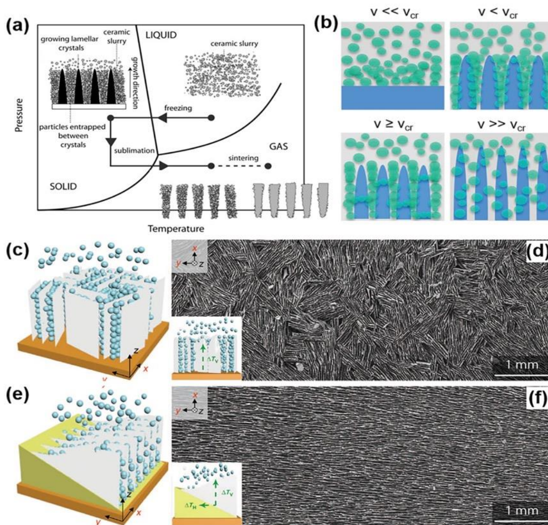
Fig. 17 Controlled oriented microstructures by freeze casting. (a) Schematic illustration of the four processing steps of freeze casting technique including slurry preparation, solidification, sublimation and post-treatment. Reproduced from ref. 240 with permission from John Wiley and Sons. (b) Schematic representation of the freezing front progression at different velocities. Reproduced from ref. 49 with permission from John Wiley and Sons. The freezing front progression is decided by the particle freezing front velocity ( v ) and the ice critical freezing front velocity ( v_{cr} ). (c) and (d) Scheme and obtained hydroxyapatite (HA) scaffold of unidirectional freezing casting with a single vertical temperature gradient ( \Delta T_v ). (e) and (f) Scheme of bidirectional freeze casting and resulting HA scaffold with both horizontal temperature gradient ( \Delta T_H ) and vertical gradient ( \Delta T_v ). Reproduced from ref. 242 with permission from American Association for the Advancement of Science.
