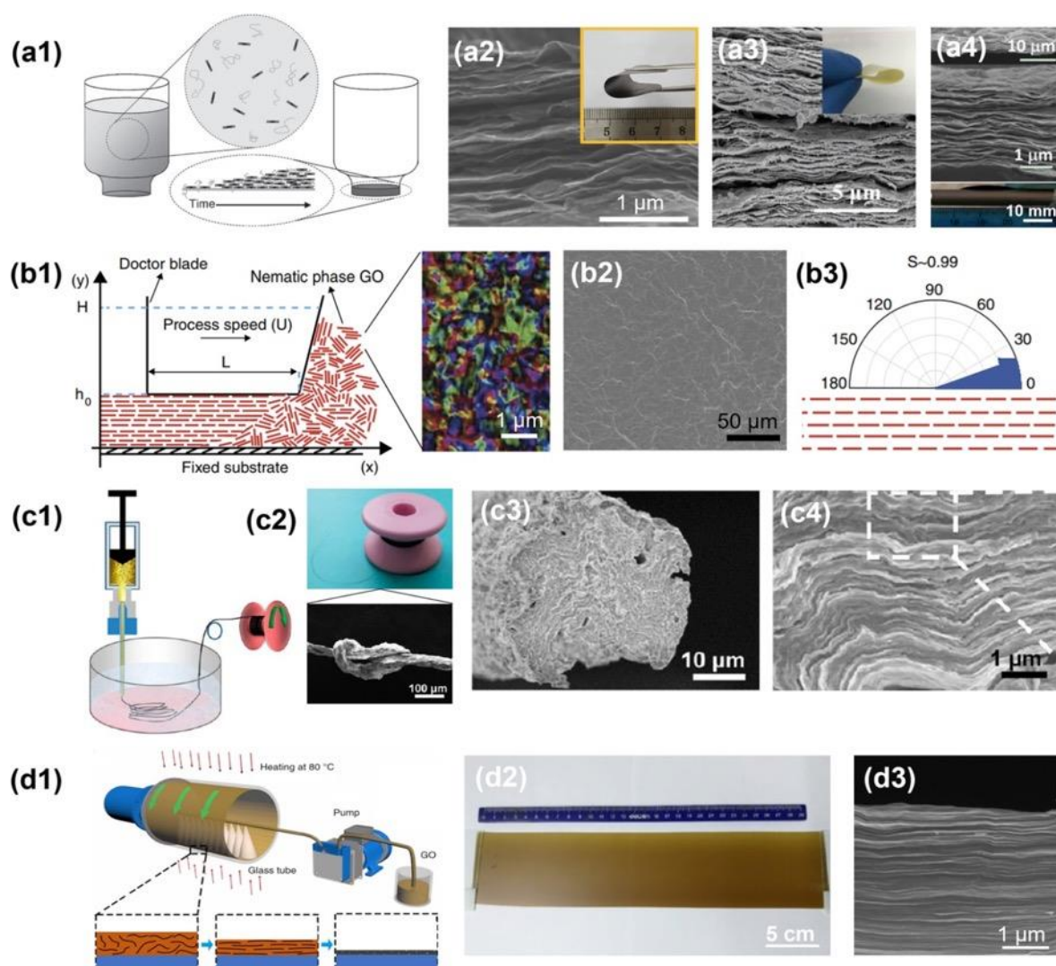
Fig. 7 Horizontal alignment of 2D materials assisted by mechanical force. (a1) Schematic representation of the vacuum-assisted filtration of nano-composite films. Reproduced from ref. 129 with permission from John Wiley and Sons. (a2) SEM image showing cross section of the horizontally aligned MXene membrane. Reproduced from ref. 134 with permission from Springer Nature. (a3) SEM image of aramid nanofiber (ANF)/BNNS film with tightly packed microstructure. Reproduced from ref. 146 with permission from John Wiley and Sons. (a4) Cross-sectional SEM images of flexible free-standing \text{Ti}_3\text{C}_2\text{T}_x/\text{PDDA} films. Reproduced from ref. 133 with permission from National Academy of Science. (b1) Schematic of tape casting processing of nematic graphene oxide (GO). (b2) SEM image showing top surface of the shear-aligned GO membrane. (b3) Organization of graphene sheets in membranes. Reproduced from ref. 137 with permission from Springer Nature. (c1) Schematic representation of wet spinning for polyacrylonitrile-grafted GO (GO-g-PAN) fibers and (c2) fabricated GO-g-PAN fibers. (c3) and (c4) Cross-sectional SEM images of GO-g-PAN3 fibers with horizontally aligned layers. Reprinted with permission from ref. 139. Copyright (2013) American Chemical Society. (d1) Schematic of the continuous centrifugal casting process. (d2) A GO film with a dimension of \sim 30 \times 10 \text{ cm}^2 and a thickness of \sim 100 \mu\text{m} . (d3) SEM image of a GO film showing highly aligned and compact layered structure. Reproduced from ref. 57 with permission from Springer Nature.
