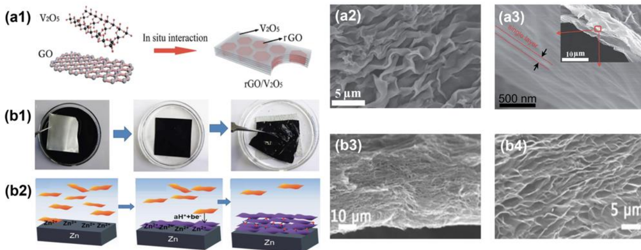
Fig. 8 Horizontal alignment of 2D materials by bottom-up approach. (a1) Schematics of the hydrothermal fabrication process of rGO/V_2O_5 hybrid sheets. (a2) Top view SEM image of rGO/V_2O_5 hybrid sheets showing a wrinkled surface. (a3) The cross-section SEM image showing individual layers. Reproduced from ref. 155 with permission from Royal Society of Chemistry. (b1) Schematic representation of the interfacial gelation mechanism where a Zn foil (in grey) is immersed in a GO dispersion (black). (b2) Graphene gelation mechanisms at the surface of the metallic foil. (b3) and (b4) Morphologies of the graphene aerogels. Reproduced from ref. 158 with permission from John Wiley and Sons.
