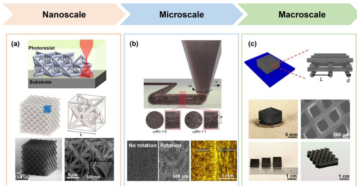
Fig. 19 Integration of materials into nanoscale, microscale and macroscale by 3D printing. (a) Fabrication of nano-sized hollow-tube alumina ceramic nanolattices using two-photon lithography. Reproduced from ref. 258 with permission from American Association for the Advancement of Science. (b) Carbon fiber orientation during printing through the rotational direct ink writing with fiber alignment controllable in micro scale. Reproduced from ref. 259 with permission from National Academy of Science. The helical pattern is dictated by the rotational rate ( \omega ), translational velocity ( v ), surface fiber orientation ( \phi ) and dimensionless rotation rate ( \omega R/v ). (c) 3D printed graphene aerogel microlattices with various structures and dimensions up to centimeter scale. Reproduced from ref. 260 with permission from Springer Nature.
