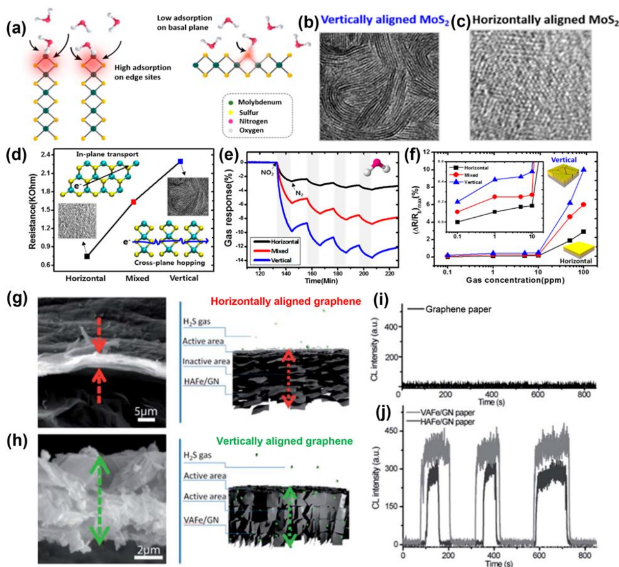
Fig. 4 Gas adsorption properties of MoS 2 films with horizontal, vertical and mixed alignment for gas sensing. (a) Schematic illustration showing mechanism of gas adsorption on edge sites and basal plane of MoS 2 films. SEM images of (b) vertically aligned and (c) horizontally aligned MoS 2 films. (d) Resistance in relation to different alignment with higher resistance in vertically aligned MoS 2 film because of cross-plane hopping of carriers. (e) Resistance changes of 100 ppm NO 2 gas adsorption demonstrate the superior gas sensing properties of edge sites than basal plane. (f) Maximum electrical responses of the synthesized MoS 2 films within 0.1-100 ppm of NO 2 exposure. Reprinted with permission from ref. 55. Copyright (2015) American Chemical Society. Morphologies of (g) horizontally aligned Fe 2 O 3 /graphene paper and (h) vertically aligned Fe 2 O 3 /graphene paper. Response curves of H 2 S on chemiluminescence (CL) intensity of (i) graphene paper fabricated by traditional filtration and (j) vertically arranged Fe 2 O 3 /graphene nanosheets (VAFe/GN) and horizontally arranged Fe 2 O 3 /graphene nanosheets (HAFe/GN) with controlled orientation. Reproduced from ref. 87 with permission from Royal Society of Chemistry.
