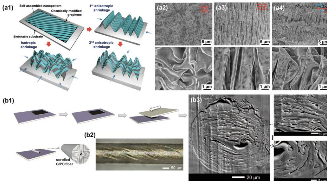
Fig. 13 Heterogeneous graphene nanostructures created by (a) crumpling and (b) scrolling. (a1) Schematic illustration of crumpling for self-assembled nanopattern. SEM images of (a2) isotropically, (a3) uniaxially, and (a4) hierarchically crumpled graphene with different shrinkage directions specified in read arrows. Reproduced from ref. 59 with permission from John Wiley and Sons. (b1) Schematic illustration of scrolling graphene/polycarbonate (G/PC) nanocomposite. (b2) Optical microscope image of the scrolled fiber. (b3) Cross-sectional SEM images of the scrolled fiber. Reproduced from ref. 163 with permission from American Association for the Advancement of Science.
