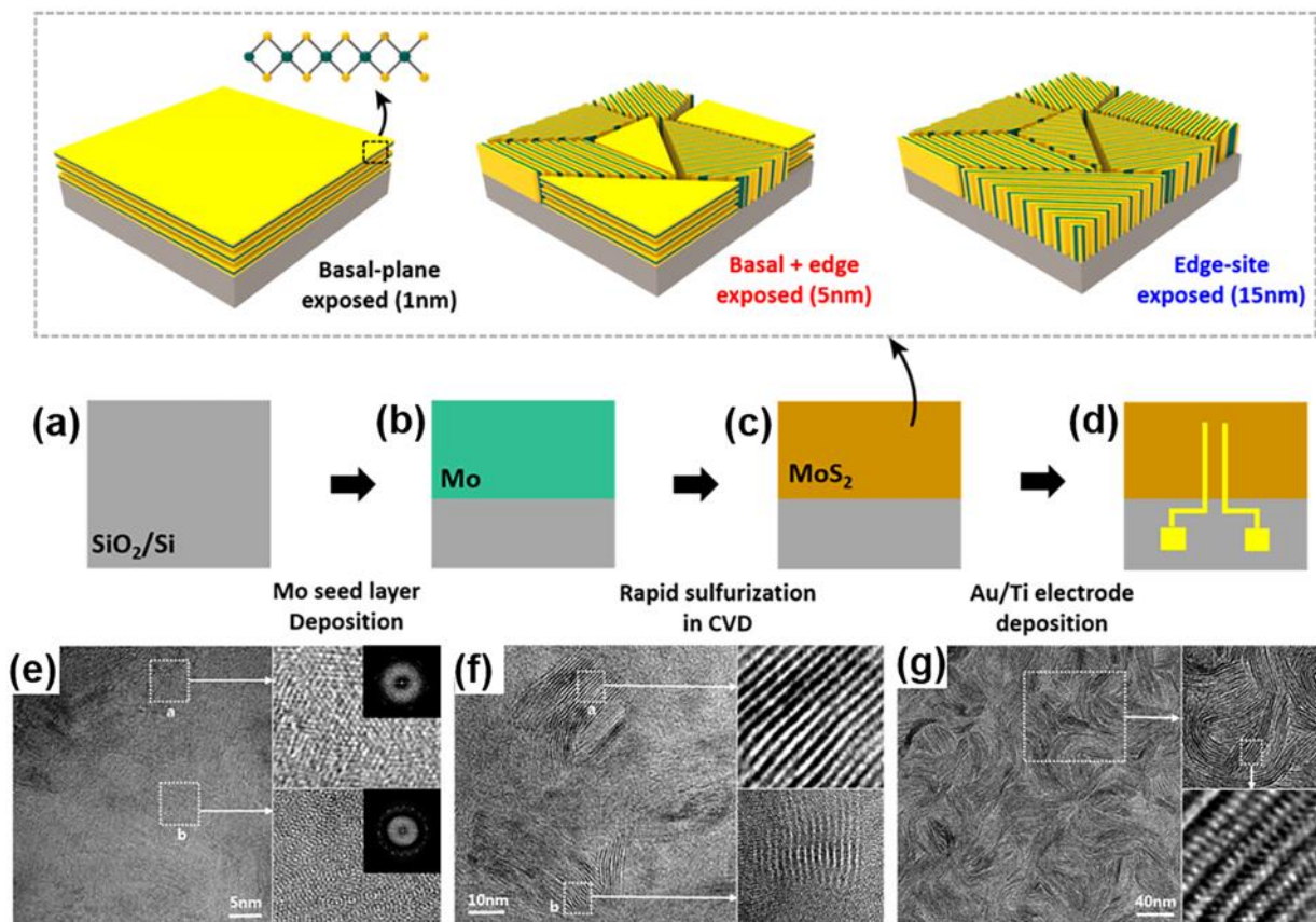
Fig. 18 Controlled orientation of 2D MoS 2 films by CVD growth. (a) and (b) Mo seed layers are predeposited on substrate. (c) Growth of MoS 2 films from horizontal to vertical alignment upon increasing Mo seed layer thickness. (d) Deposition of Au/Ti electrode for application. (e) Horizontal layer alignment from 1 nm seed thickness. (f) Horizontal and vertical heterogeneous alignment from 5 nm seed thickness. (g) Vertical film alignment grown from 15 nm seed layer thickness. Reprinted with permission from ref. 55. Copyright (2015) American Chemical Society.
