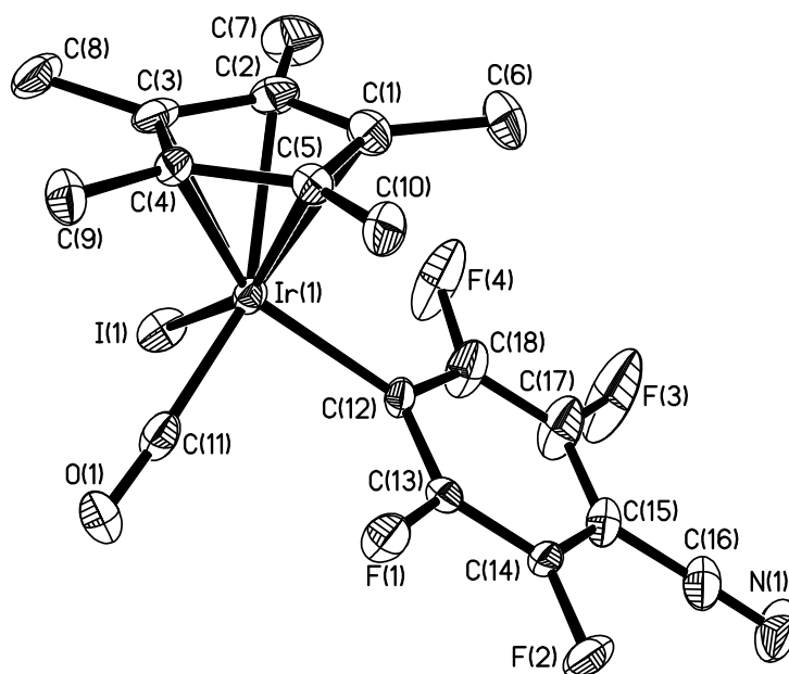
Figure 2. ORTEP plot of 6b showing the atomic numbering scheme, with thermal ellipsoids drawn at 50% probability level and hydrogen atoms omitted for clarity. Selected bond lengths (Å) and angles (deg): Ir(1)-I(1) = 2.6967(5); Ir(1)-C(11) = 1.891(7); Ir(1)-C(12) = 2.084(6); O(1)-C(11) = 1.108(8); C(16)-N(1) = 1.122(9); C(15)-C(16) = 1.441(9); C(12)-Ir(1)-I(1) = 91.58(16); C(11)-Ir(1)-C(12) = 91.9(2).
