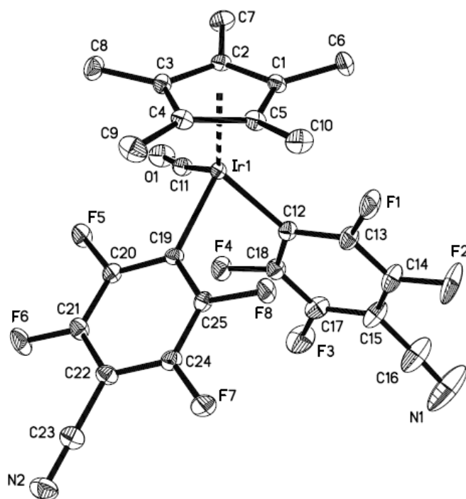
Figure 1. ORTEP plot of 4 showing the atomic numbering scheme, with thermal ellipsoids drawn at 50% probability level and hydrogen atoms omitted for clarity. Selected bond distances [Å] and angles [deg]: Ir(1)-C(11), 1.866(4); Ir(1)-C(19), 2.068(3); Ir(1)-C(12), 2.095(3); C(11)-Ir(1)-C(19), 97.24(14); C(11)-Ir(1)-C(12), 90.42(15); C(19)-Ir(1)-C(12), 84.00(12).
