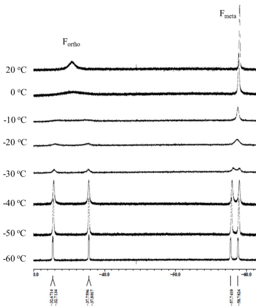
Figure 3. Variable temperature ^{19}\text{F} NMR spectra of 6a .
