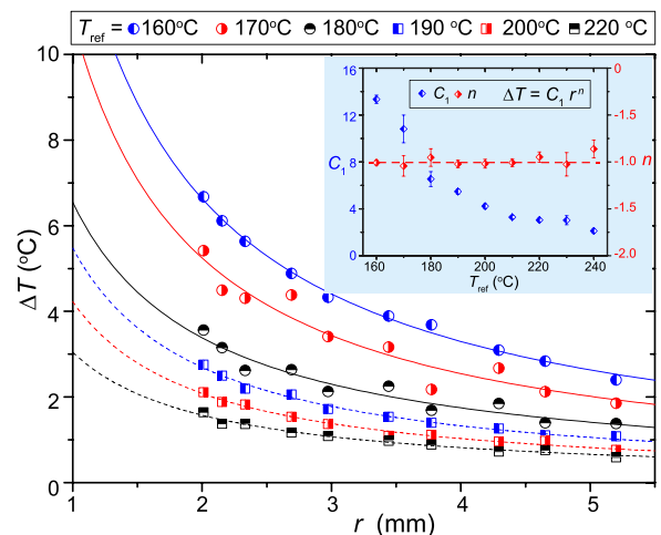
FIG. 2. The variations of the temperature difference in terms of the radius from the stagnation point. The temperature profiles follow the spherical conductive heat transfer pattern \Delta T = C_1 r^{-1} . The inset shows the fitting constants.
