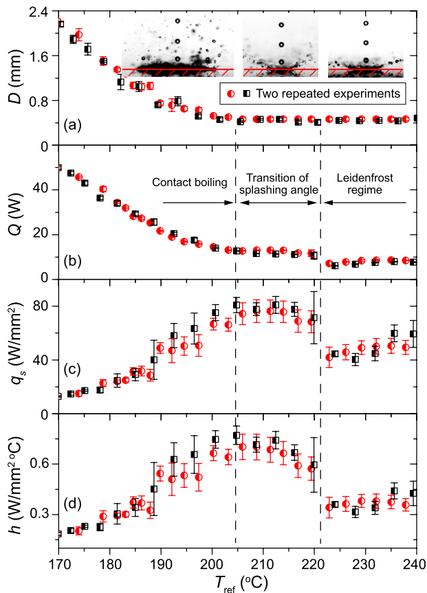
FIG. 4. The variations of (a) wetted diameter captured by the high-speed camera, (b) cooling power, (c) solid-liquid interface heat flux, and (d) heat transfer coefficient. All the experiments are repeated twice. The insets demonstrate the hydrodynamic patterns in three different regimes.
