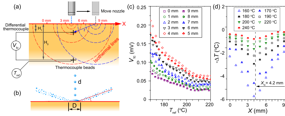
FIG. 1. (a) The experimental method. A differential thermocouple measures the temperature difference (converted from the voltage output) between the two points below the top surface. The temperature of the lower point is measured using a separated thermocouple as the reference. After each set of measurements, the surface is cooled down and the nozzle is horizontally shifted by 1 mm to conduct the next set. (b) A stable wetted area, with a diameter D , could be established at the high substrate temperatures. 6 (c) The variations of the voltage output of the differential thermocouple when the droplet train impinges onto different locations of the copper substrate. (d) The temperature differences measured by the differential thermocouple. A sunken point in the middle of the surface is observed.
