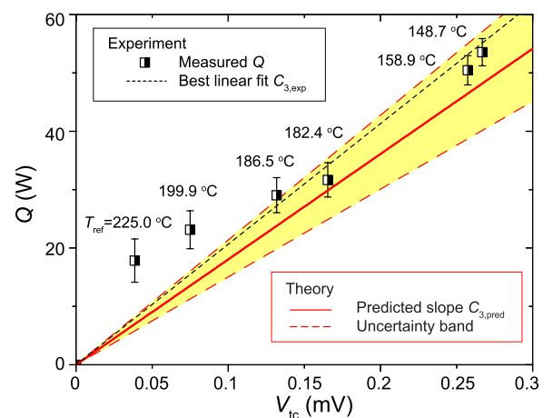
FIG. 3. The cooling power against the voltage output of the differential thermocouple. The coefficient, C_3 , is obtained by two mean values, namely, the theoretically predicted C_{3,pred} and the experimentally calibrated C_{3,exp} .
