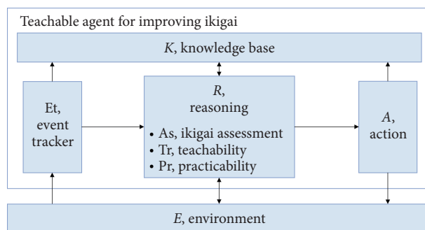
Fig. 1 Teachable agent for improving ikigai architecture.
