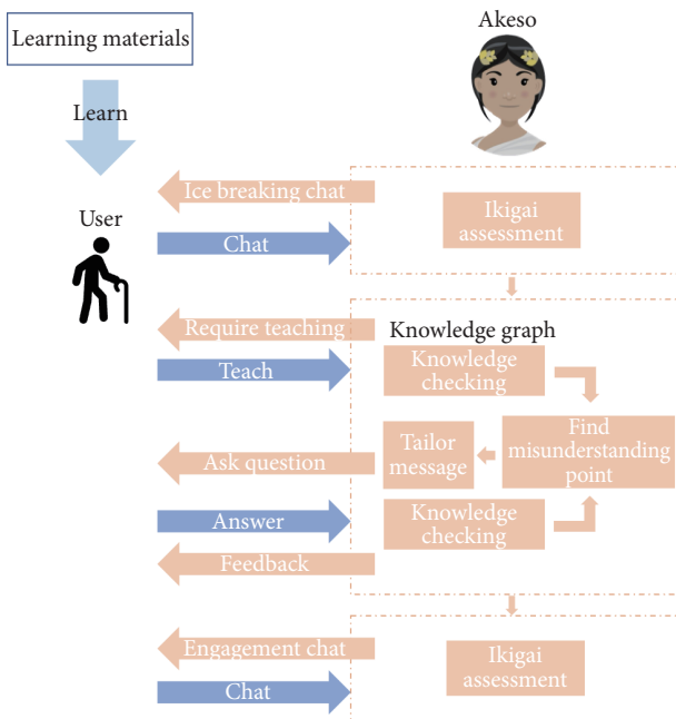
Fig. 4 Akeso conversation flow.
