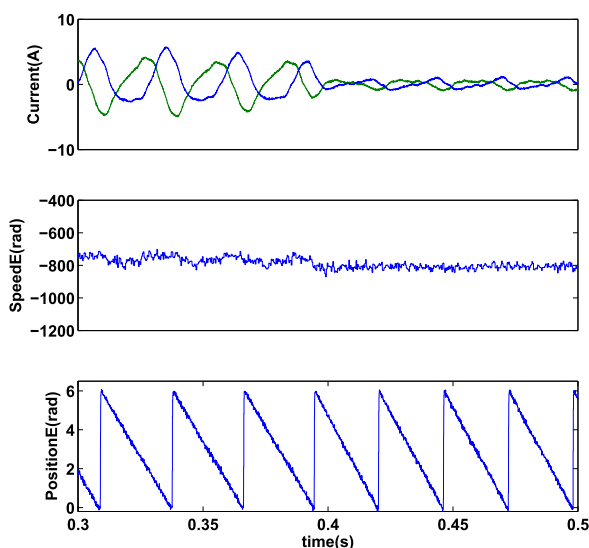
FIGURE 12. 9 Nm unload dynamic performance of sensorless control based on SMO at 800 rpm speed.
