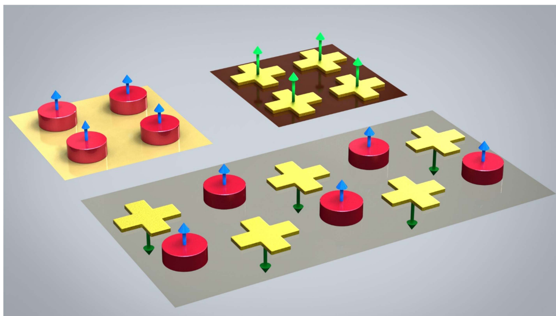
Figure 1. Schematic of the magnetic dipole ordering in electromagnetic metasurfaces. On the upper part two generic metasurfaces composed of the arrays of different elements (meta-atoms) exhibit a FM or AFM ordering depending on the distance between elements, when magnetic dipole moments are induced. Being combined together, two dissimilar types of meta-atoms with the FM ordering can create an AFM ordering with the staggered structure of optically-induced magnetic dipole moments. The structure is one of several possible realizations of the AFM order. The other type of element ordering is shown e.g. in figure 1 in [7].
