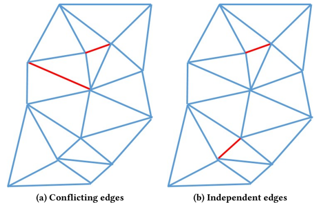
Figure 2: An illustration of conflicting edges (a) and independent edges (b).
