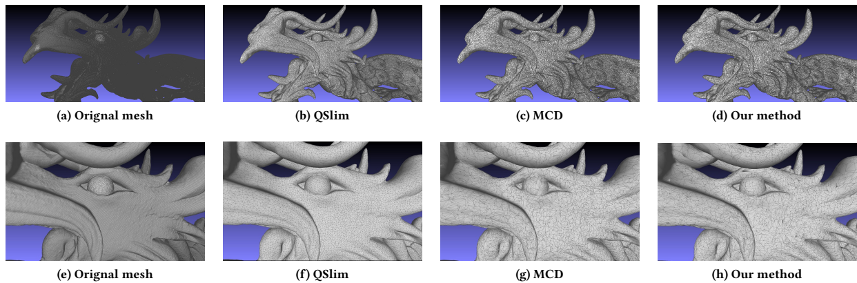
Figure 4: Comparison of the simplification results for the dragon model.
