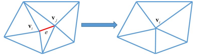
Figure 1: A demonstration of edge collapse. Edge e(v_i, v_j) (red) is collapsed into one vertex v_c .
