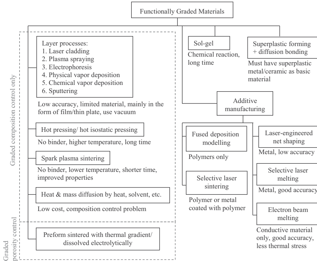
Figure 1. Summary of various FGM fabrication techniques
