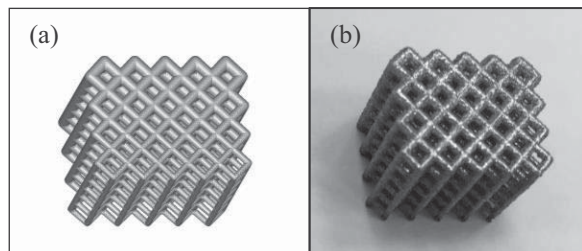
Figure 2. (a) FGM design in software, (b) FGM fabricated by SLM technique
