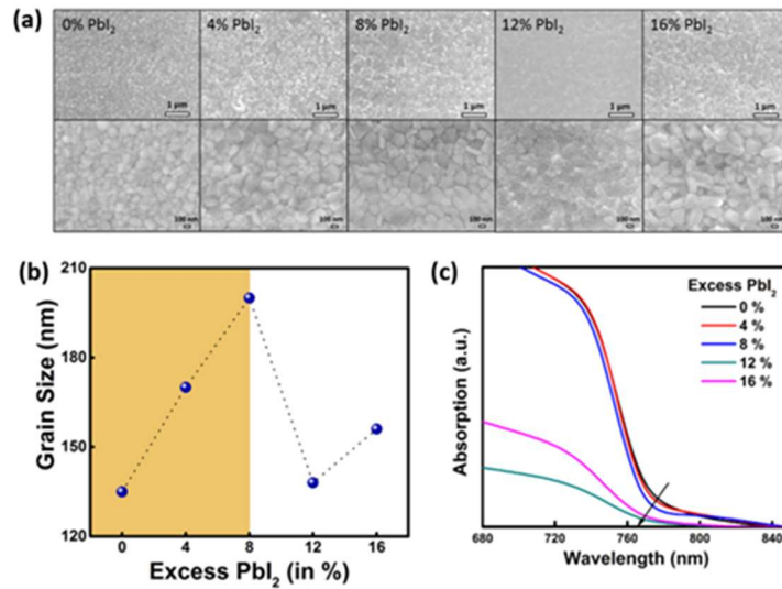
Figure 4. (a) Top view SEM micrographs of the perovskite films having different amount of initial \text{PbI}_2 concentrations, corresponding high-resolution images are in the bottom of the image. (b) Average grain size estimated from the SEM analysis as function of \text{PbI}_2 percentage and (c) UV-Vis optical absorption spectra for the pristine fresh films with varying initial \text{PbI}_2 concentrations.
