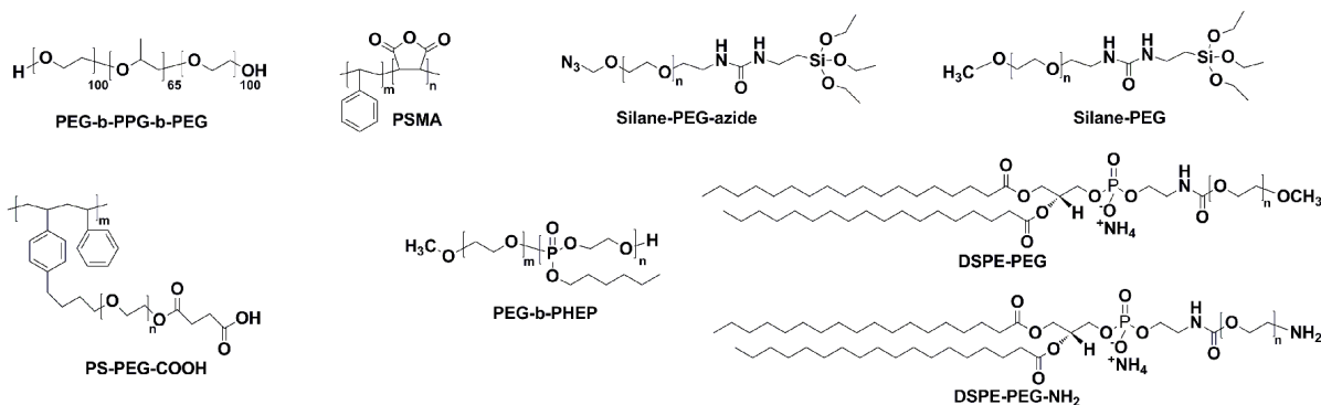
Scheme 3. Chemical structures of amphiphilic polymers used for imaging and phototherapy in living mice.
