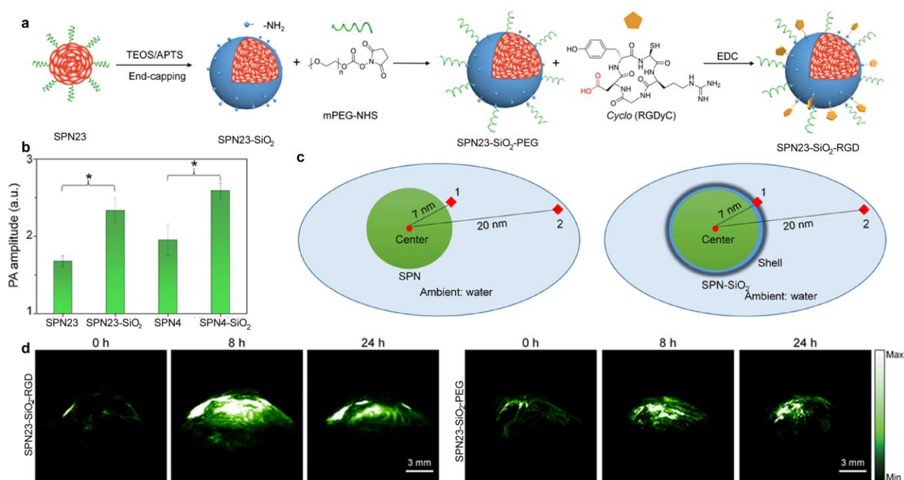
Fig. 9. (a) Synthesis of SPN23-SiO 2 -PEG and SPN23-SiO 2 -RGD. (b) Comparison of PA amplitudes of SPN23 and SPN23-SiO 2 at 760 nm, and SPN4 and SPN4-SiO 2 at 680 nm under the same concentration. (c) Schematic illustration of the COMSOL simulation for SPNs. (1 and 2 are the two test points for measuring temperature and PA signal). (d) Representative PA images of subcutaneous
