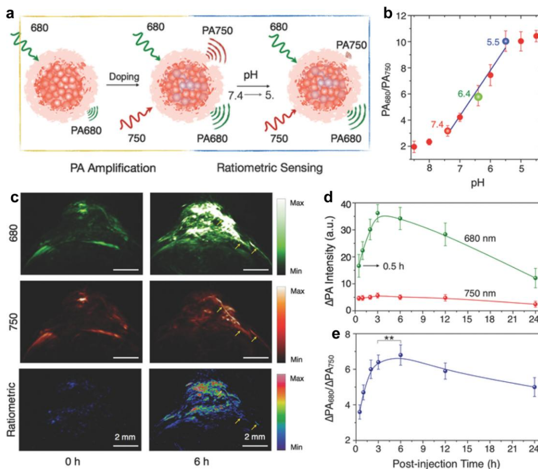
Fig. 12. (a) Schematic illustration of doping-induced PA amplification and pH-sensing mechanism. (b) Quantification of the ratiometric PA signal ( PA_{680}/PA_{750} ) of SON750 at different pH. The blue line represents linear fitting from pH = 7.4 to 5.5. (c) PA and ratiometric images ( \Delta PA_{680}/\Delta PA_{750} ) of a subcutaneous HeLa tumor in a nude mouse before and at 6 h after intravenous administration of SON750. The representative PA MIP images with axial view are demonstrated. The yellow arrows indicate one of the blood vessels of the tumor. (d) Quantification of the PA intensity increment at 680 nm and 750 nm. (e) The ratiometric PA signal ( \Delta PA_{680}/\Delta PA_{750} ) as a function of time post-injection of SON750. The first set of data readout was conducted at 0.5 h post-injection. The pulsed laser was tuned to 680 or 750 nm for PA imaging. Reprinted with permission from Ref. [142], copyright 2016, WILEY-VCH Verlag GmbH & Co. KGaA, Weinheim.
