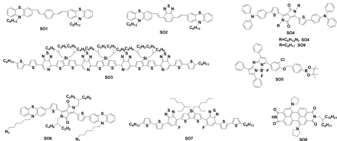
Scheme 2. Chemical structures of SOs used for imaging and phototherapy in living mice.
