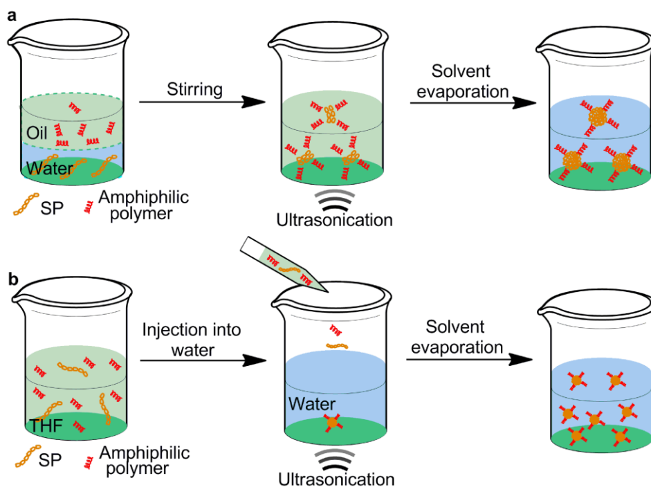
Scheme 4. Schematic representation of mini-emulsion (a) and nanoprecipitation (b) methods for the preparation of SPNs.
