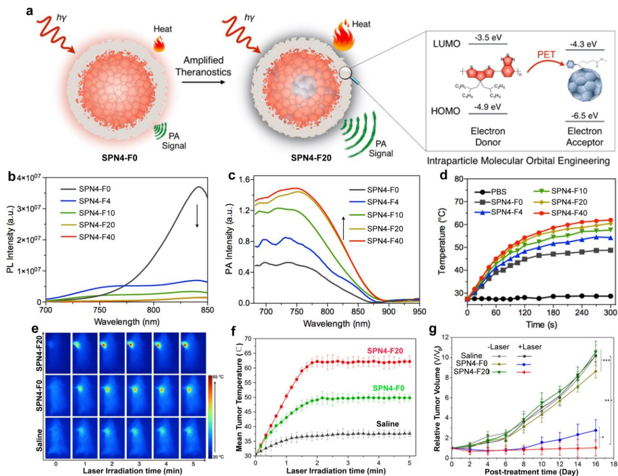
Fig. 15. (a) Illustration of photo-induced electron transfer induced amplified theranostic SPN4-F20. The highest occupied molecular orbital (HOMO) and lowest unoccupied molecular orbital (LUMO) are -4.9 and -3.5 eV for SP4 and -6.5 and -4.3 eV for PC70BM, respectively. (b) Photoluminescence (PL) and (c) PA spectra of SPN4. The arrows indicate the decrease (b) or increase (c) of the intensities with the increased doping amount of PC70BM in SPN4. (d) The temperature of SPN4 solutions as a function of laser irradiating time at the power intensity of 0.5 \text{ W/cm}^2 . (e) Thermal images of 4T1 tumor-bearing mice under 808 \text{ nm} laser irradiation ( 0.3 \text{ W/cm}^2 ) after administration of saline, SPN4-F0, or SPN4-F20 at post-injection time of 6 \text{ h} . (f) Mean tumor temperature as a function of laser irradiation time after the systemic administration of saline, SPN4-F0, or SPN4-F20 at 6 \text{ h} post-injection. (g) Tumor growth curves of different groups of mice after systemic treatment with saline, SPN4-F0 or SPN4-F20 with and without laser irradiation. Reprinted with permission from Ref. [116], copyright 2016, American Chemical Society.
