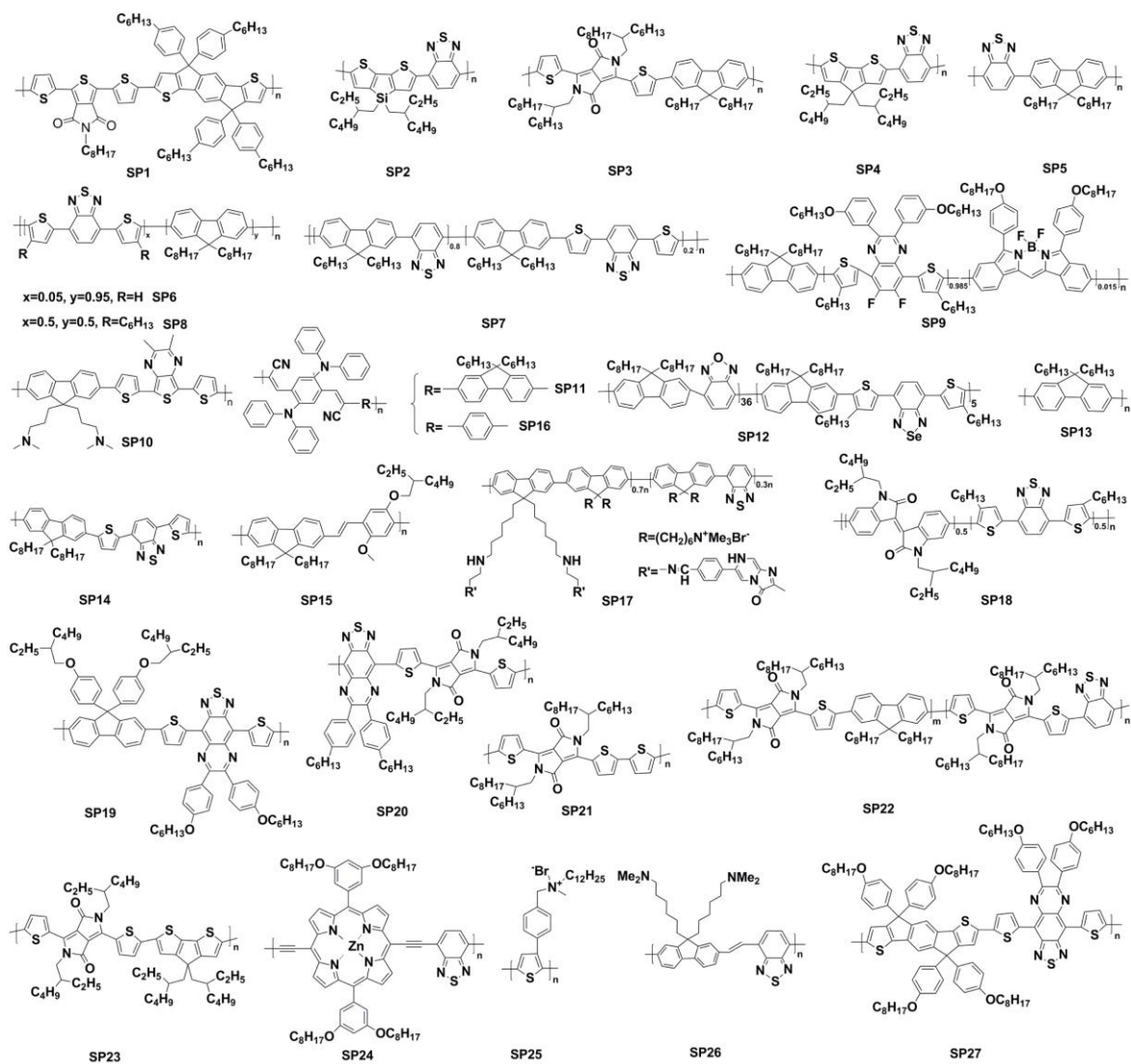
Scheme 1. Chemical structures of SPs used for imaging and phototherapy in living mice.
