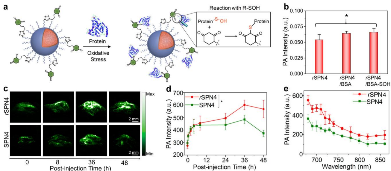
Fig. 13. (a) Illustration of the mechanism of the specific reaction between rSPN4 and BSA-SOH. (b) PA intensities at 680 nm of rSPN4 and rSPN4 in the presence of BSA or BSA-SOH. (c) The representative PA maximum intensity projection images with axial view of tumor at representative time-points after administration of rSPN4 or SPN4 via tail vein injection. (d) Quantification of PA as a function of time post-injection of rSPN4 or SPN4. (e) Real-time in vivo PA spectra of tumor at the post-injection time of 48 h. The PA data were acquired at 680 nm. Reprinted with permission from Ref. [147], copyright 2016, American Chemical Society.
