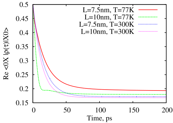
FIG. 1. Real part of an off-diagonal density matrix element with respect to time, demonstrating that the coherence survives for over 100 ps even at 77 K. The graphs are shown for two regimes: a strong coupling L = 7.5 nm and a moderate coupling L = 10 nm.
