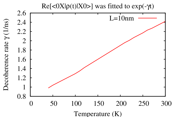
FIG. 2. The decoherence rate in a pair of interacting QDs calculated as a linear fit of \text{Re}[\langle 0X|\rho(t)|X0\rangle] \sim \exp(-\gamma t) . The typical decoherence rate remains at 1 \text{ ns}^{-1} scale. Calculated for d = 3.3 nm and L = 10 nm using 200 ps overaging window.
