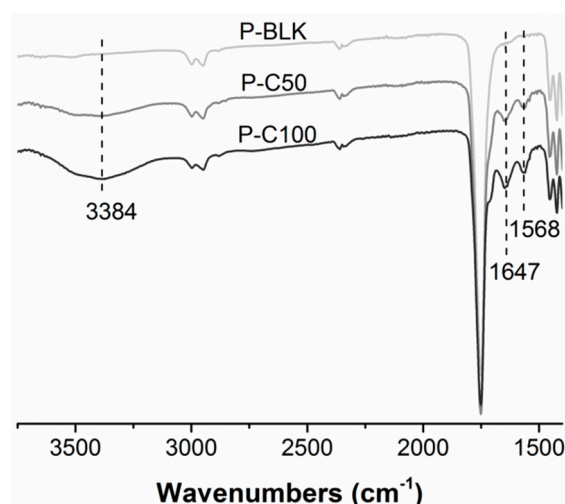
Figure 2. Attenuated total reflection Fourier transform infrared spectroscopy (ATR-FTIR) analysis of P-BLK (light gray), P-C50 (gray), and P-C100 (black).
