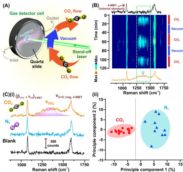
Figure 3. Remote SERS-based gas detector. (A) Scheme showing remote tracking of CO 2 in real time for several cycles with multilayered Ag@MOF platform. (B) Time-resolved SERS intensity profile of 1360 cm -1 band, showing the absorption and detection of CO 2 in several cycles. (C)(i) Spectroscopic observation of CO 2 vibrational modes (shown with respect to internal standard peak of 4-MBT embedded on the particle) in the detection of CO 2 , which is not observed in the control experiments with N 2 flow and no gas (blank), (ii) Principle component analysis (PCA) score plot of stand-off spectra observed in the presence of CO 2 and N 2 .
