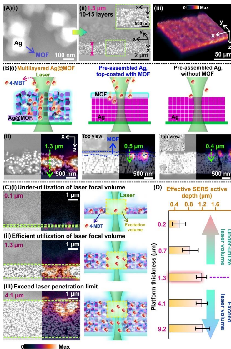
Figure 1. 3D MOF-SERS platform. (A)(i) SEM image showing Ag@MOF particles, (ii) cross-sectional SEM image showing the side view of multilayered Ag@MOF platform and (iii) 3D x-y-z SERS image of a segment of the platform (performed with 20× confocal objective lens). (B)(i) Schemes and (ii) cross-sectional SEM images showing the structure and how airborne molecules are absorbed and detected in different platform configuration. Half of the images in (ii) are overlapped with x-z SERS hyperspectral images (with 100× objective lens) showing the penetration of gaseous 4-MBT into the platform (Ag in the platforms has no 4-MBT surface groups prior to exposure). (C)(left) SEM images overlapped with x-z SERS
