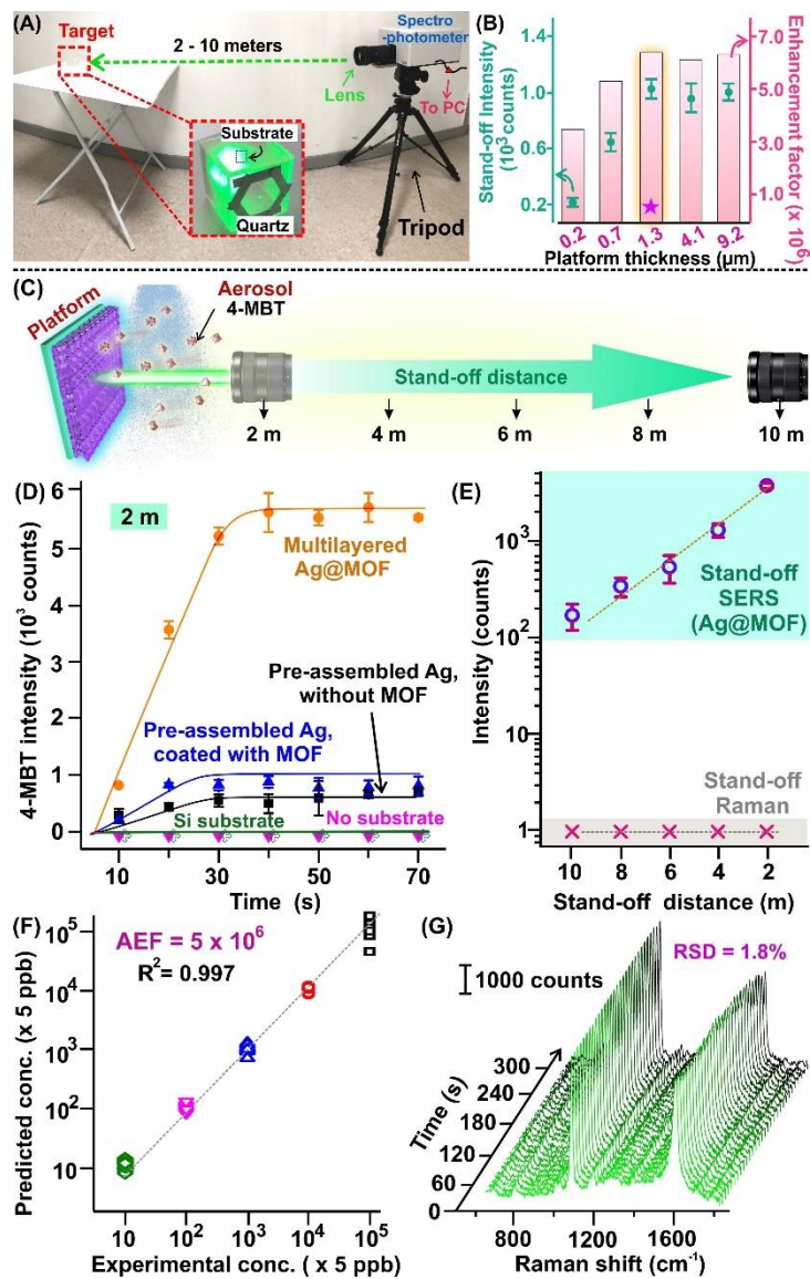
Figure 2. Stand-off SERS with 3D MOF-SERS platform (A) Set-up of our stand-off SERS system. (B) Stand-off intensity (at 2 m) of 4-MBT's 1077\text{ cm}^{-1} obtained from platforms of thickness ranges from 0.2 - 9.2\ \mu\text{m} (with Ag pre-functionalized with 4-MBT). (C) Scheme showing the stand-off SERS detection of aerosolized 4-MBT (500 ppm, Ag in the platforms has no 4-MBT surface groups). (D) Real-time 4-MBT intensity obtained in the stand-off SERS detection using different platforms. (E) 4-MBT intensity obtained at distances from 2 to 10 m using our A@MOF SERS platform and normal Raman detection. (F) Partial least square
