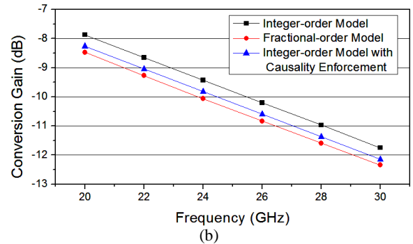
Fig.12. Conversion gain of mixer when input signal at 95~105 GHz down converted to 20~30 GHz with LO frequency of 75 GHz.
