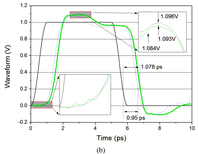
Fig.9. Impulse responses of T-line models under different input waveforms: (a) sinusoidal input, (b) piecewise-Linear input.
