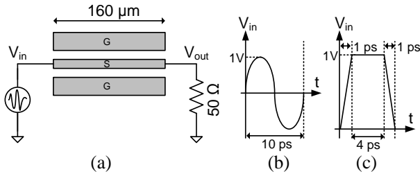
Fig.8. (a) Schematic of T-line impulse response simulation, (b) Waveform of sinusoidal input, (c) Waveform of trapezoidal input.
