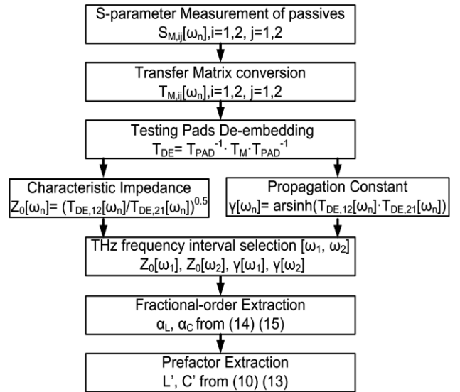
Fig.2. Fractional-order T-line modeling parameters extraction flow.
