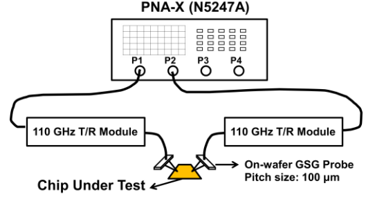
Fig.5. Measurement setup of on-wafer S-parameter testing up to 110GHz.
