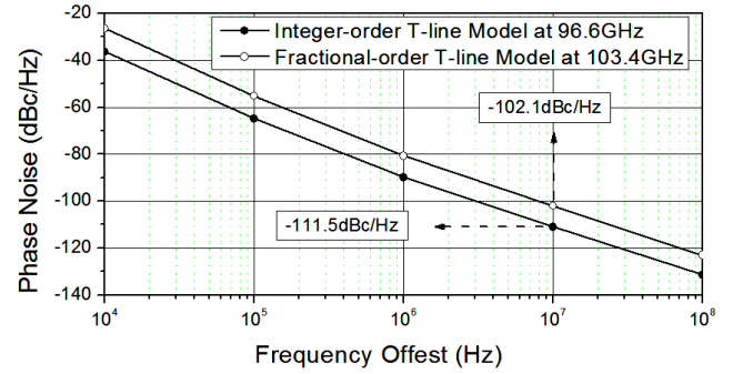
Fig.15. Phase noise of standing-wave oscillators with T-line modeled the fractional-order and integer-order models.
