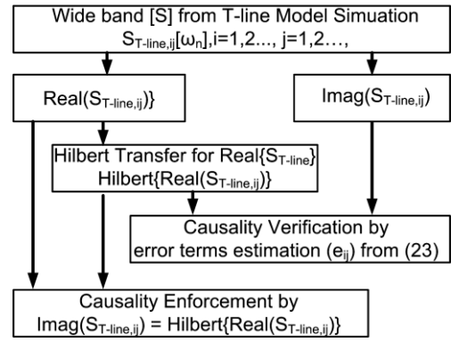
Fig.3. Causality verification and enforcement flow.
