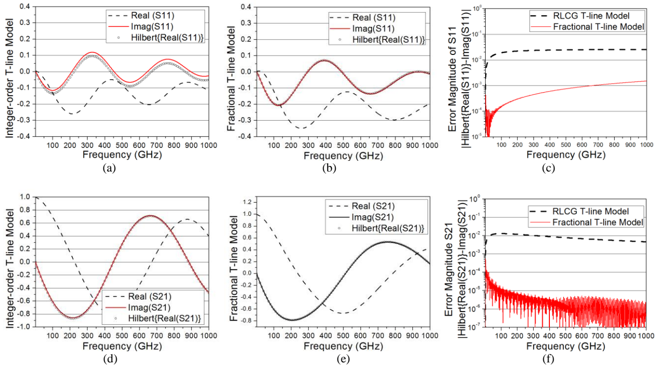
Fig.7. Causality verification by Hilbert transformation for both integer and fractional order T-line models: (a) integer-order T-line model S11; (b) fractional-order T-line model S11; (c) error magnitude comparison of S11; (d) integer-order T-line model S21; (e) fractional-order T-line model S21; and (f) error magnitude comparison of S21.
