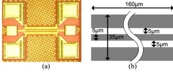
Fig.4. (a) Die photo of T-line, (b) Dimensions of T-line.
