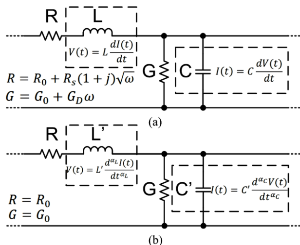
Fig.1. RLGC unit-cell equivalent circuits of T-line: (a) integer-order model; and (b) fractional-order model.
