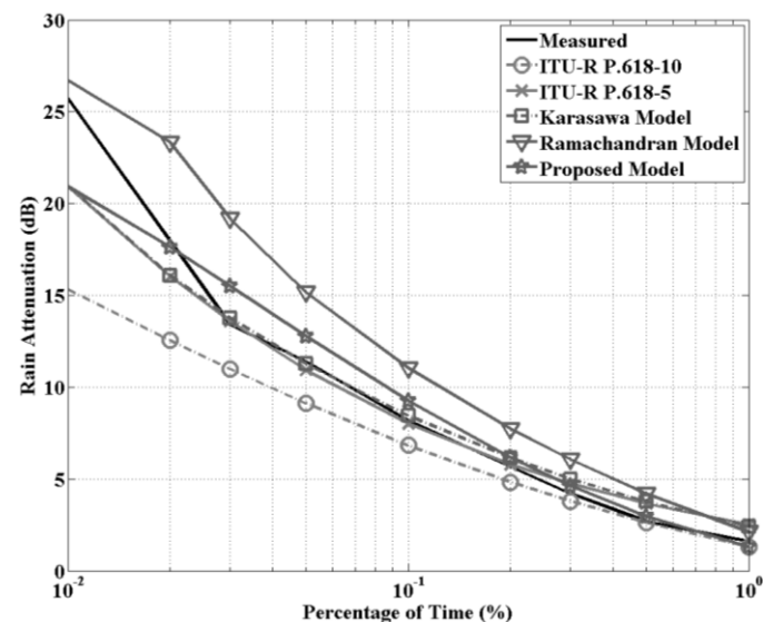
Fig. 7. CCDF of Rain Attenuation at Cameroon ( F = 11.6 GHz; \theta = 47^\circ ).
