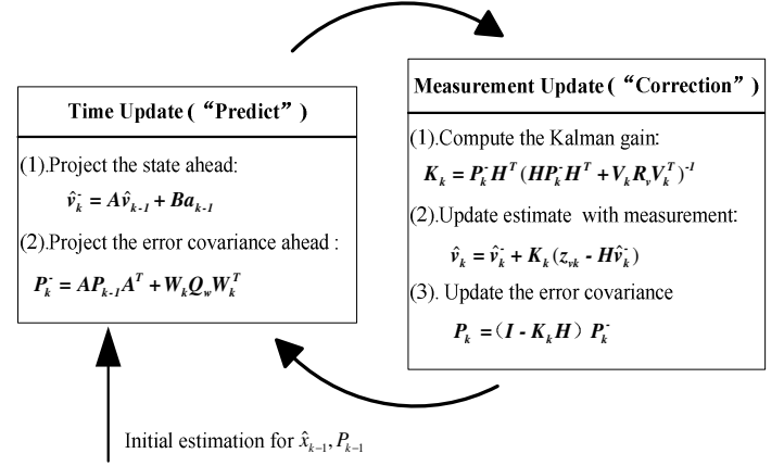
Figure 5: Velocity tracking Kalman filter
