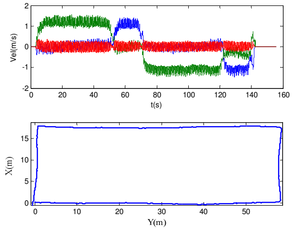
Figure 14: Outdoor localization
