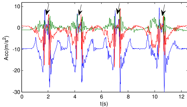
Figure 17: Root Accelerometer measurement while jumping
