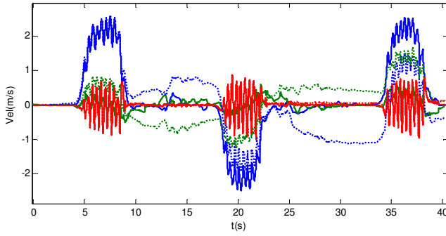
Figure 15: Jogging velocity
