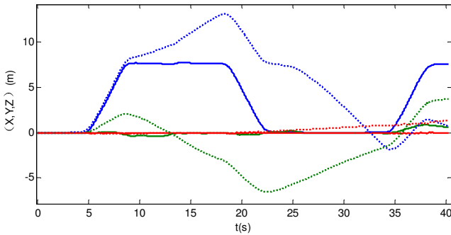
Figure 16: Jogging localization
