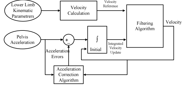
Figure 2: Velocity Tracking Algorithm
