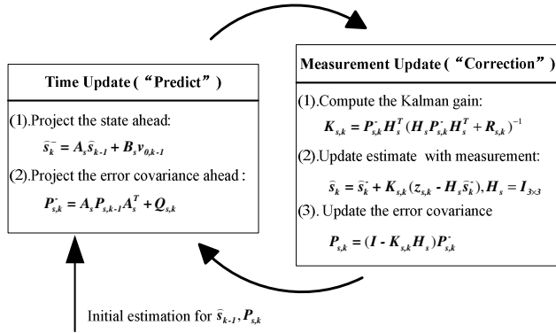
Figure 8: Localization Kalman filter in V-SLAC
