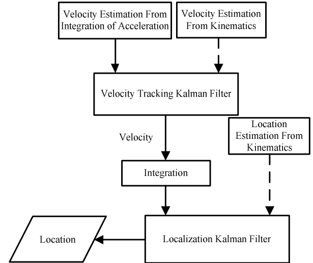
Figure 6: Fusion algorithm for localization
