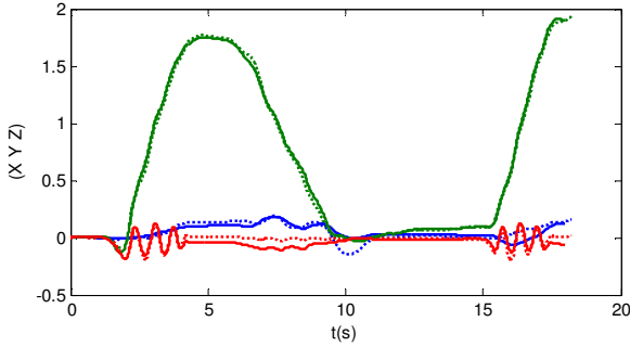
Figure 12: Benchmark study of A-SLAC: root position
