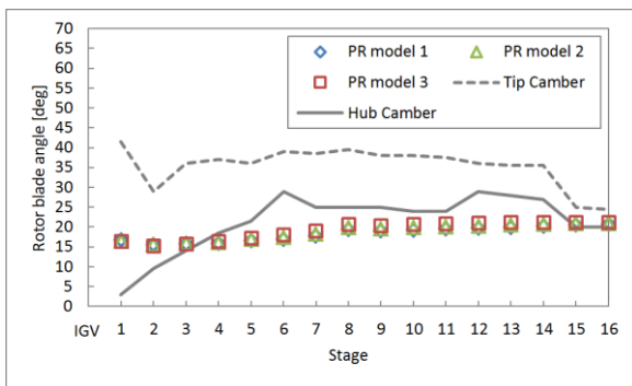
(A) Rotor blade angle
