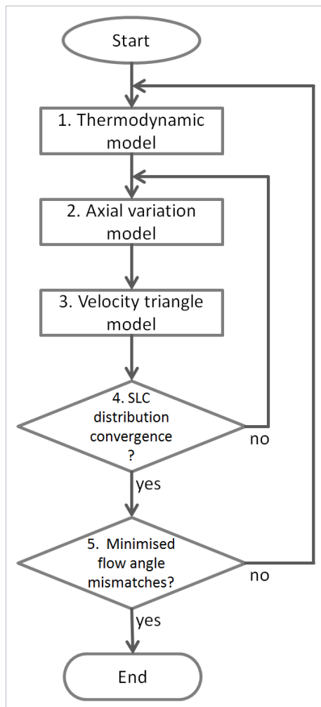
Figure 1. Overview of the stage un-stacking method
