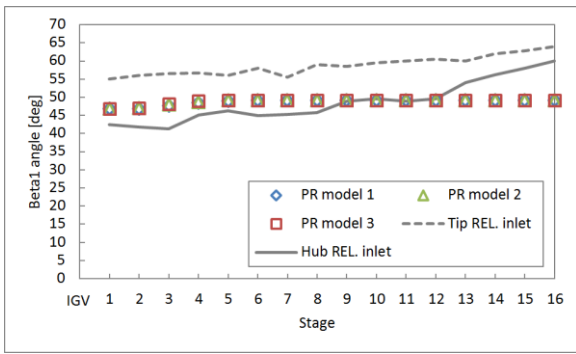
(A) Stage \beta_1 flow angle
