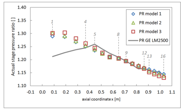
(B) Actual stage pressure ratio
