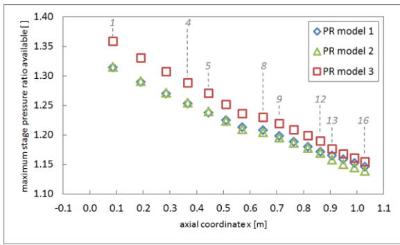
(A) Maximum available stage pressure ratio
