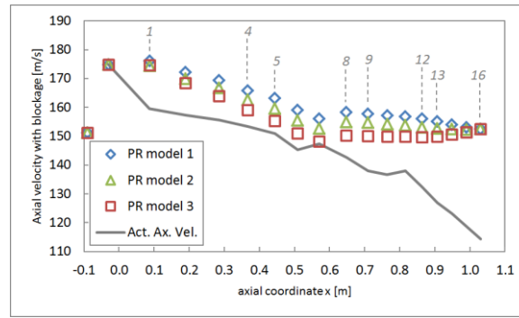
Figure 8. Stage axial velocity with different pressure ratio models (stage outlets indicated by numbers in italics)
