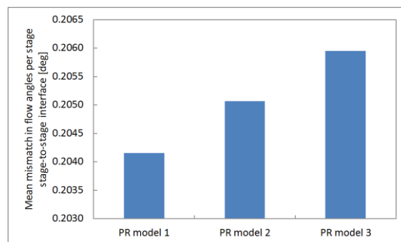
Figure 6. Comparison of mean flow angle mismatch between pressure ratio models
