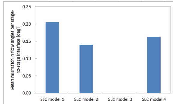
Figure 11. Comparison of mean flow angle mismatch between SLC models
