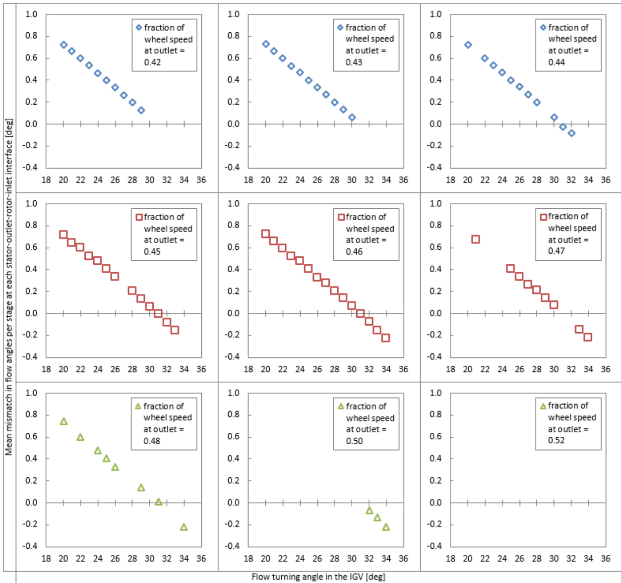
Figure 4. The effect of flow turning angle in the IGV on the mean mismatch in flow angles per stage at each stator-outlet-rotor-inlet interface
