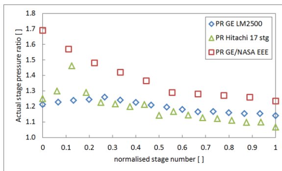
Figure 16. Pressure ratio distribution of selected gas turbines
