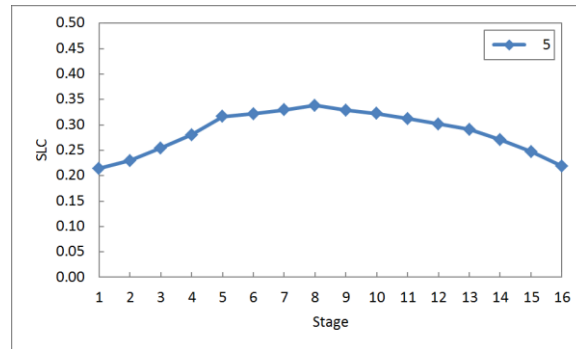
Figure 17. Estimated SLC distribution for the compressor in the LM 2500 gas turbine
