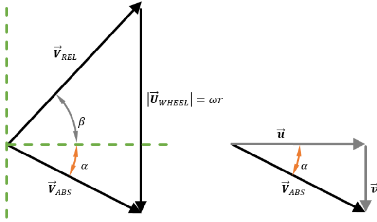
Figure 2. Velocity diagram at the rotor inlet and rotor outlet
