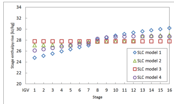
Figure 13. Specific stage static enthalpy rise with different SLC models
