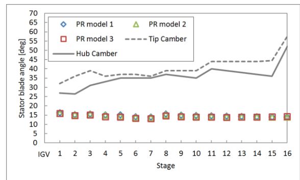
(B) Stator blade angle
