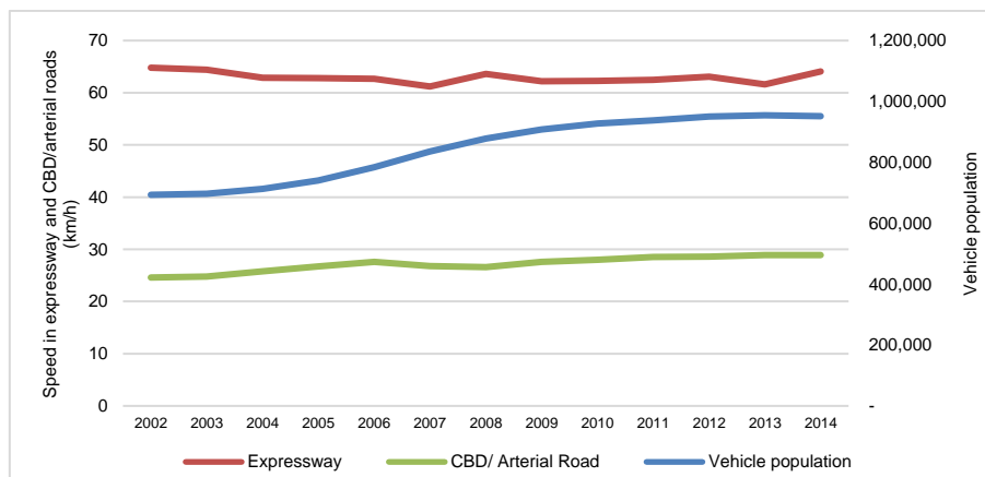
Figure 4-25: Vehicle speed vs vehicle population (adopted from (LTA 2015))
