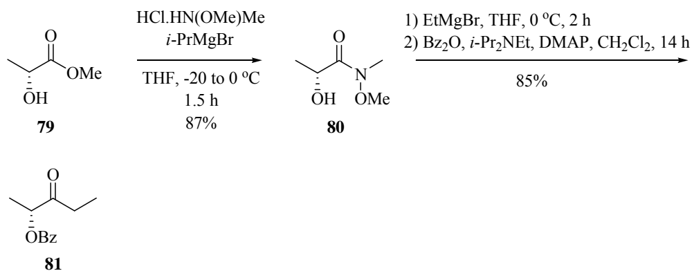
Scheme 2.2 Synthesis of subunit 81
