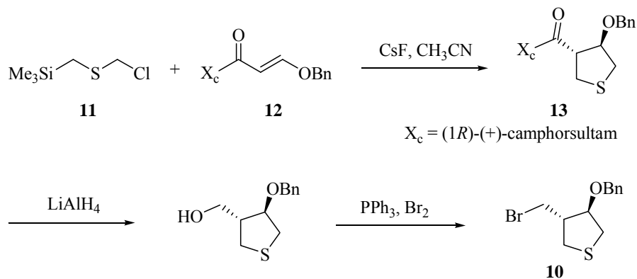
Scheme 1.4 Synthesis of enantiopure tetrahydrothiophene building block 10
