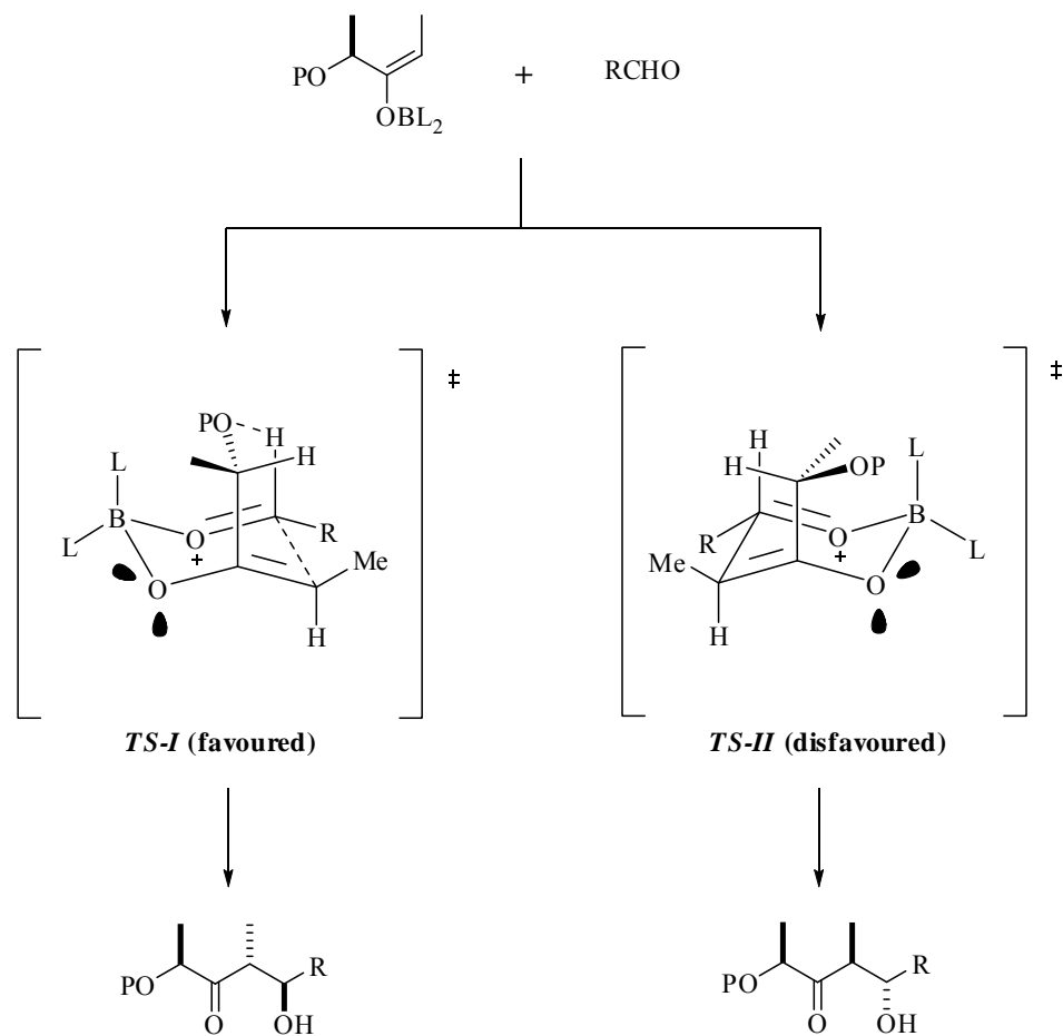
Scheme 2.6 Two possible chair transition states for aldol reaction
