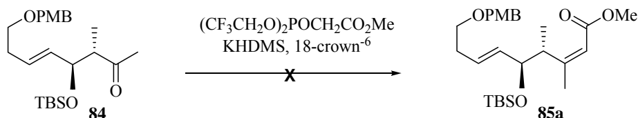
Scheme 2.8 Failed attempt to synthesis of 85a
