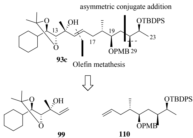
Scheme 3.6 The olefin metathesis strategy between precursors 99 and 110
