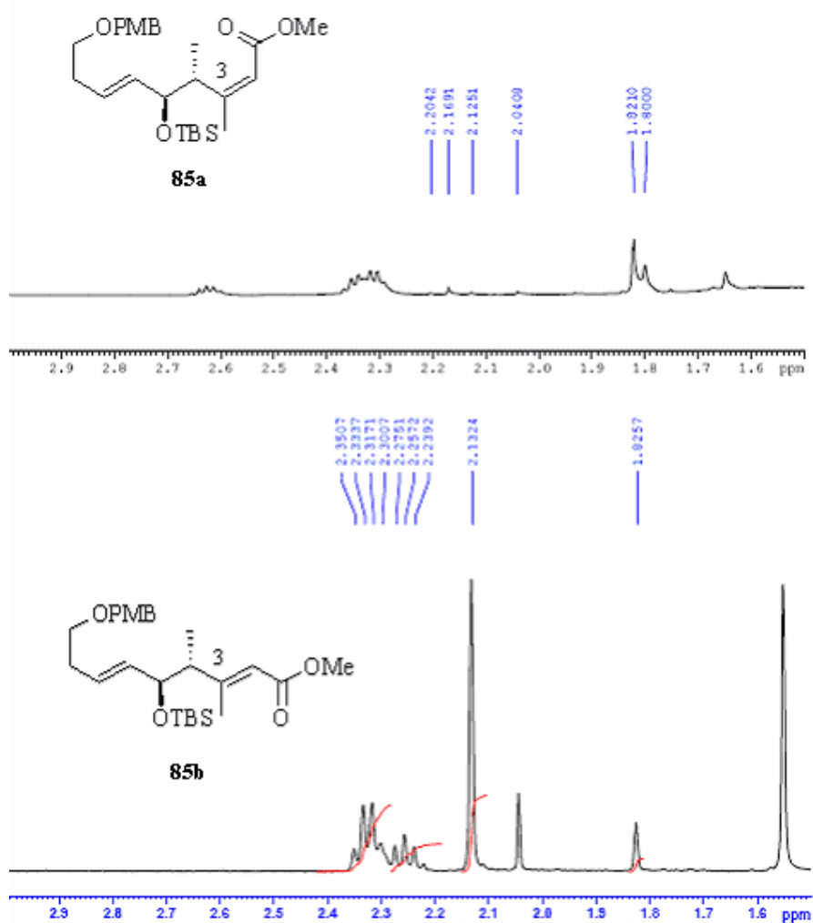
Figure 2.1 Comparison 1 H NMR spectra of 85a and 85b
