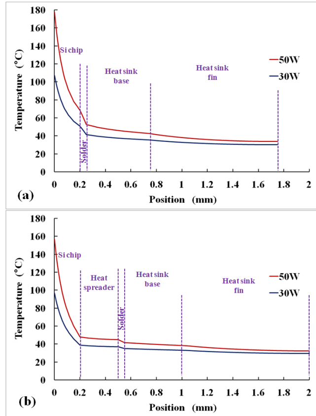
Fig.9 Temperature profile (vertical across the structure for (a) model without diamond heat spreader and (b) with it.
