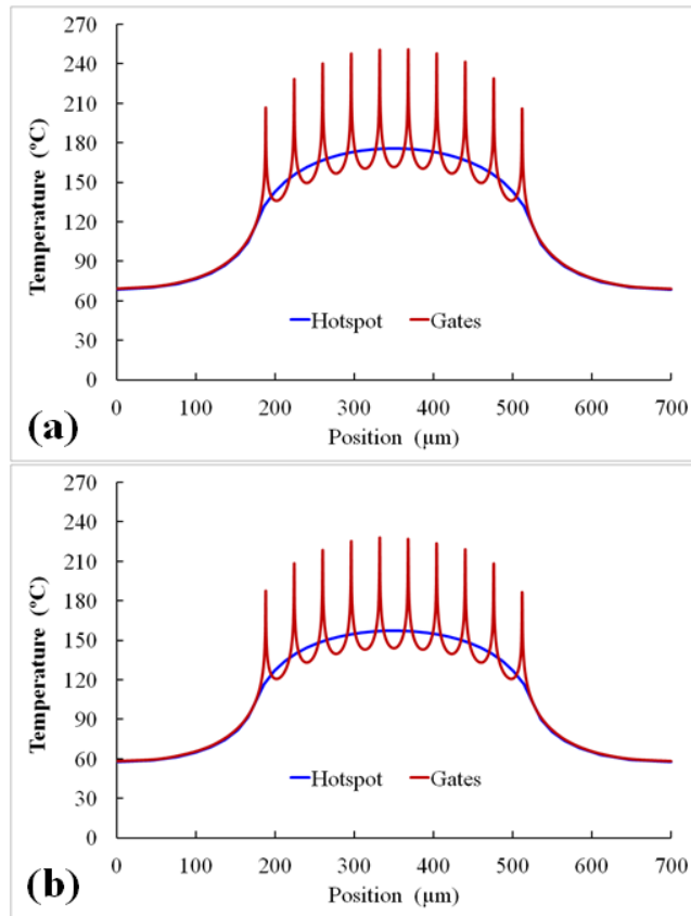
Fig.11 Temperature profile in the longitudinal direction along 10 gate fingers of (a) structure without diamond heat spreader and (b) with diamond heat spreader.
