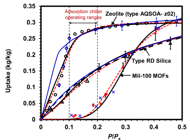
FIG. 1. Adsorption characteristics of various hydrophilic and hydrophobic porous adsorbents with adsorption cooling operating ranges. Here, the red dotted lines (---) indicate the DA isotherm model, the blue lines (—) define the isotherms models of BET theory, and the black dotted lines (---) refer to Langmuir isotherm model. The proposed adsorption uptake modeling (—) agrees well with experimental data ( \pm 5\% error). Langmuir and BET fail to fit with the experimental data of S-shaped isotherms.
