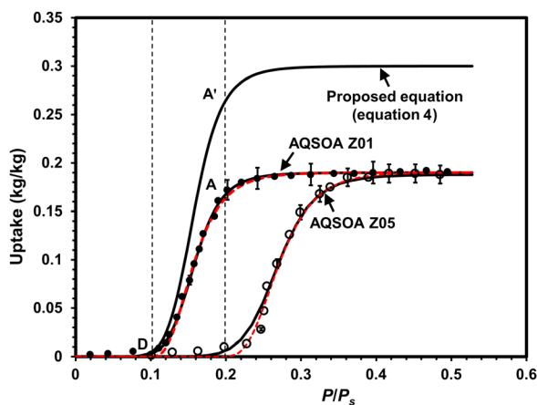
FIG. 2. Water vapor uptakes on AQSOA-Z01 and AQSOA-Z05 with adsorption-desorption operating points. A and A' indicate adsorption and D indicates desorption. The experimental data are fitted with the proposed adsorption isotherm equation and the DA isotherm model (red dotted lines ---). Employing the proposed thermodynamic equation (4), the water vapor uptakes (—) is shown here (it can be predicted by improving the surface area and pore volume of AQSOA-Z01).
