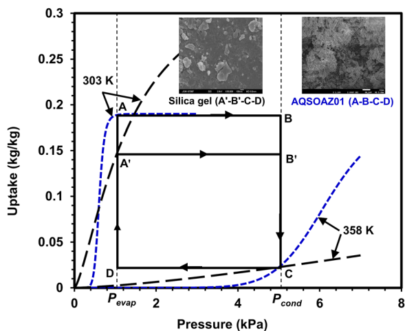
FIG. 3. Adsorption-desorption cycle of silica gel—water (A'B'CD) and AQSOA-Z01—water, where the evaporator pressure is 1 kPa and the condenser pressure is 5 kPa. The SEM pictures of silica gel and AQSOA-Z01 are shown here.
