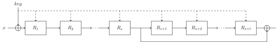
Figure 3: AES-PRF _{s,t}
