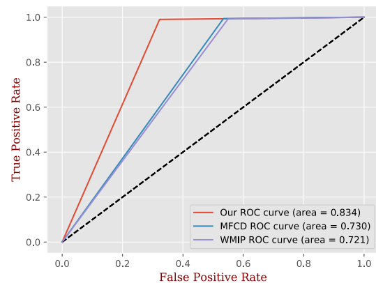
FIGURE 11. Comparison on AUC of the ROC curves.
