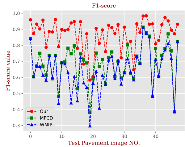
FIGURE 15. F1-score with 2-pixel vicinity of tolerance margin for each test image.
