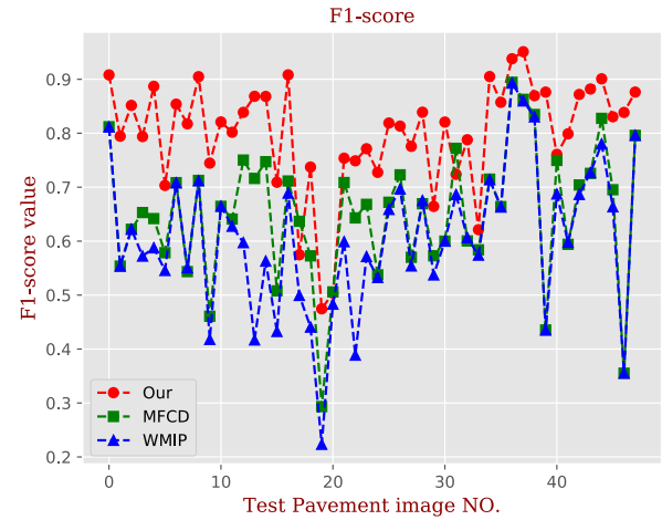
FIGURE 14. F1-score with 1-pixel vicinity of tolerance margin for each test image.
