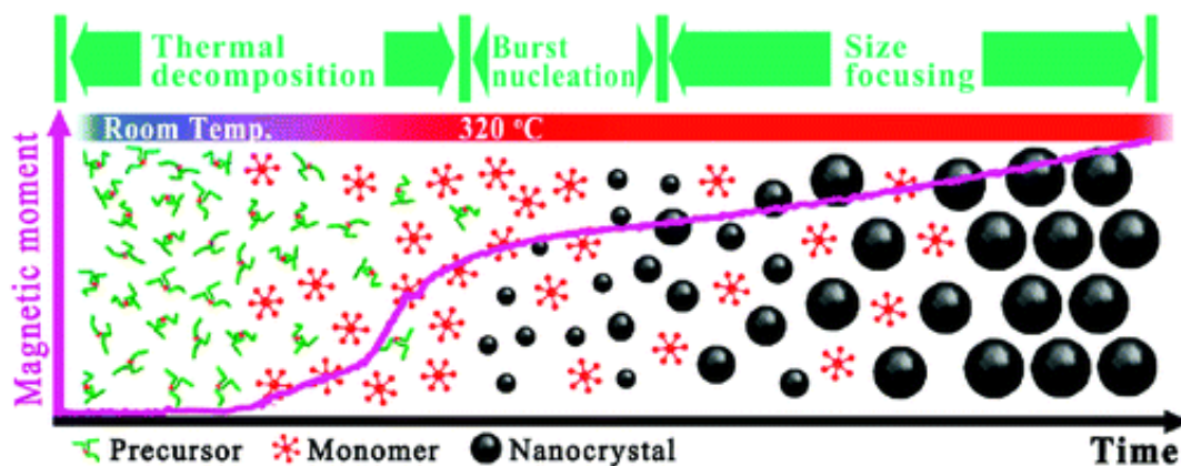
Fig. 4. Noninjection heat-up method. All precursors are present from the beginning of the reaction, and are steadily heated to initiate nucleation and growth stages. (Adapted from ref 16. Copyright 2007 American Chemical Society).
