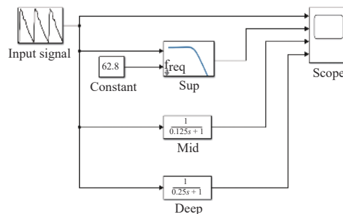
Figure 2 Simulink model for calculating perceived responses at Cun, Guan, and Chi positions
