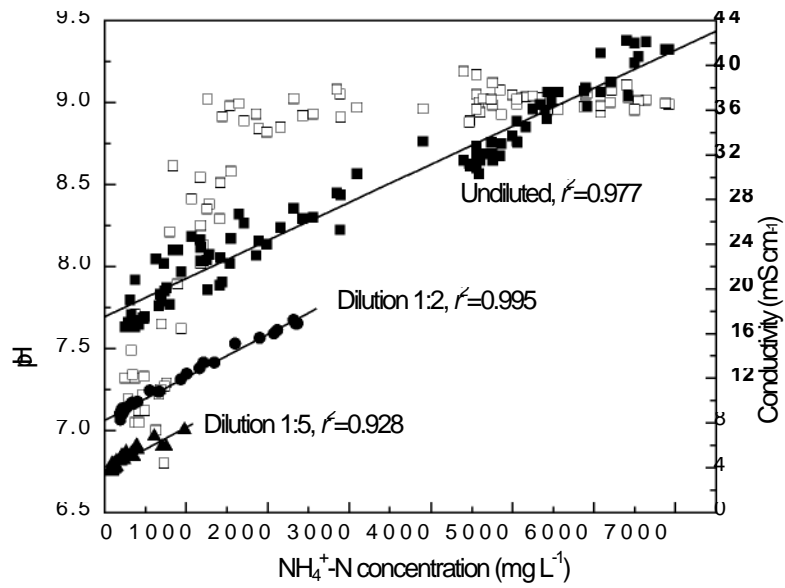
Figure 4. Correlation of pH-value ( \square ), conductivity ( \blacksquare • \blacktriangle ) and corresponding \text{NH}_4^+\text{-N} concentration during urine hydrolysis process
