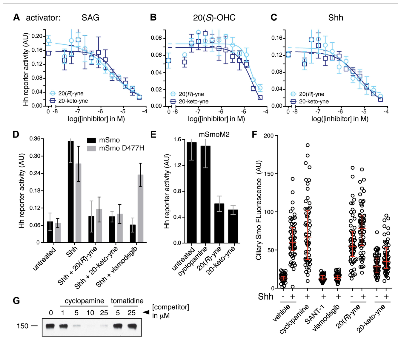
Figure 8. 20(R)-yne and 20-keto-yne can inhibit Hh signaling. (A–C) Hh reporter activation by 100 nM SAG (A), 5 μM 20(S)-OHC (B) and Shh (C) can be inhibited by both 20(R)-yne and 20-keto-yne. (D) Hh reporter activity in Smo -/- cells transfected with wild-type mSmo or mSmo D477H and then treated (48 hr) with Shh in the presence of 20(R)-yne, 20-keto-yne (both at 25 μM) or vismodegib (100 nM). (E) Hh reporter activity in NIH 3T3 cells transfected with constitutively active, oncogenic mSmoM2 and then treated (12 hr) with 20(R)-yne and 20-keto-yne (10 μM each) or cyclopamine (1 μM). (F) Accumulation of endogenous mSmo in cilia of NIH 3T3 cells treated (4 hr) with the indicated Smo ligands in the presence or absence of Shh. Each point represents the Smo fluorescence in a single cilium and the red lines denote the median and the interquartile range of mSmo fluorescence ( n = 60 for each condition). (G) The binding of mSmo CRD-Fc to 20(S)-OHC beads can be inhibited by cyclopamine but not by the structurally-related alkaloid tomatidine. Error bars denote S.D. ( n = 3).
