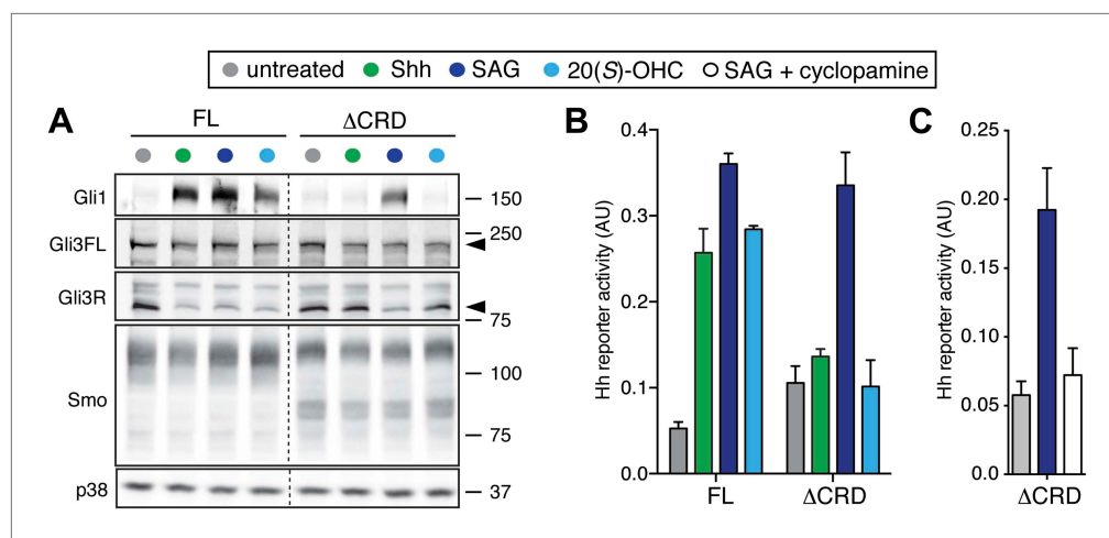
Figure 3. The mSmo CRD is required for Shh- and oxysterol-mediated activation of Hh signaling. (A) Smo -/- cells stably expressing full-length (FL) YFP-mSmo or \Delta CRD-YFP-mSmo were treated with Shh, SAG (100 nM) or 20(S)-OHC (10 \mu M). Levels of Gli1 and Gli3R protein, determined by immunoblotting after fractionation on an 8% Tris-glycine SDS-PAGE gel, were taken as a metric of pathway activation. An anti-YFP blot shows the levels of YFP-mSmo in each sample, and p38 levels are used as a loading control. (B and C) A luciferase-based Hh reporter gene was used to measure signaling in Smo -/- cells transiently transfected with constructs encoding YFP-mSmo or \Delta CRD-YFP-mSmo and then treated with the indicated Smo ligands. In (C) , \Delta CRD-YFP-mSmo activated with SAG (25 nM) can be inhibited by the co-administration of cyclopamine (5 \mu M). Error bars denote S.D. (n = 3).
