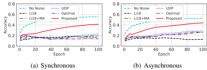
Fig. 12. The average accuracy of the agents in different modes on CIFAR10.
