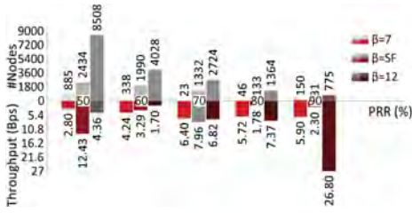
(a) Difference between LoRa and LoRaWAN in supported number of nodes and throughput for each PRR requirement.
