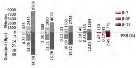
(b) Difference between LoRa and LoRaWAN in supported number of nodes and goodput for each PRR requirement.
