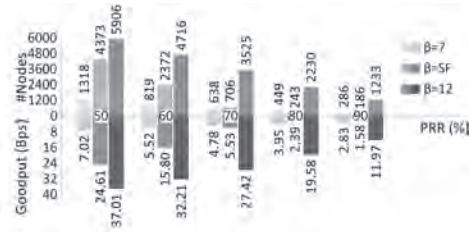
(b) Number of nodes and goodput supported by each PRR requirement.
