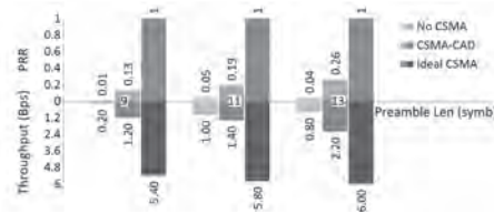
(c) PRR vs Preamble Length where payload=6B, Inter-packet Delay=15s and number of Nodes fixed to 100.
