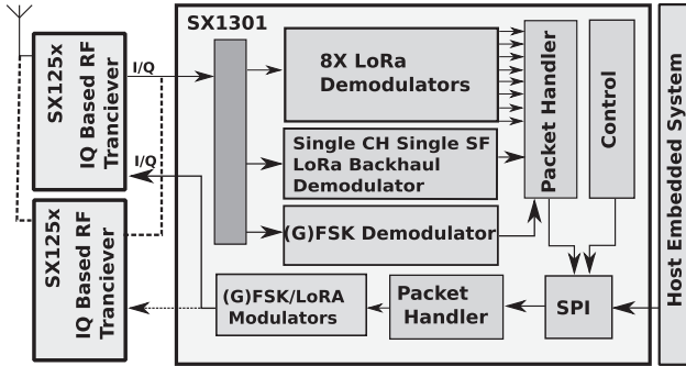
Fig. 12. Block-level overview of a LoRa SX1301 concentrator.
