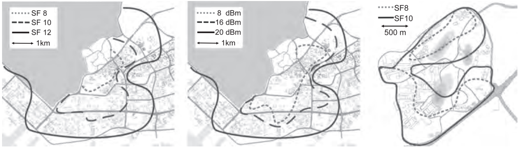
(a) Outdoor coverage with TX Pow 20dBm and varying SF. (b) Outdoor coverage with SF12 and varying TX Pow. (c) Indoor coverage with TX Pow 20dBm and varying SF.
