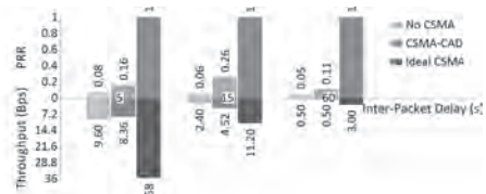
(b) PRR vs Inter-packet Delay where preamble=8, payload=6B and number of Nodes fixed to 100.
