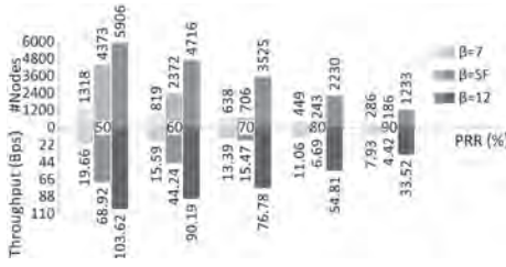
(a) Number of nodes and throughput supported by each PRR requirement.
