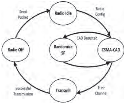
(a) The CSMA-CAD mechanism illustrated as a state diagram.
