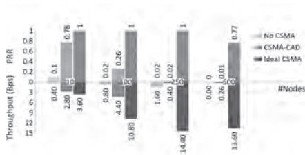
(a) PRR vs #Nodes where preamble=8, payload=6B and Inter-packet Delay fixed at 15s.
