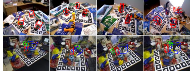
Fig. 4. The examples of pose estimation on the dataset of Tejani(the first row) and the occlusion dataset (the second row).
