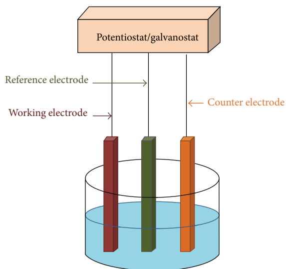
FIGURE 5: The schematic representation of the electrodeposition system [21].
