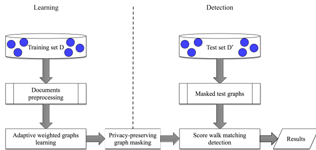
FIGURE 2. The overview of AGW.
