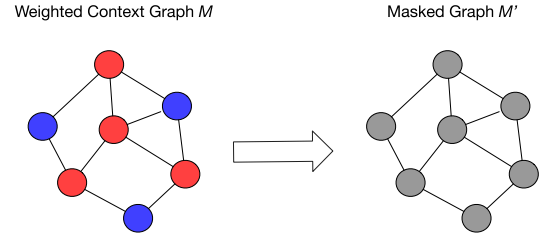
FIGURE 4. The process of graph masking.
