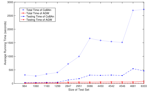
FIGURE 11. The running time of CoBAn and AGW.
