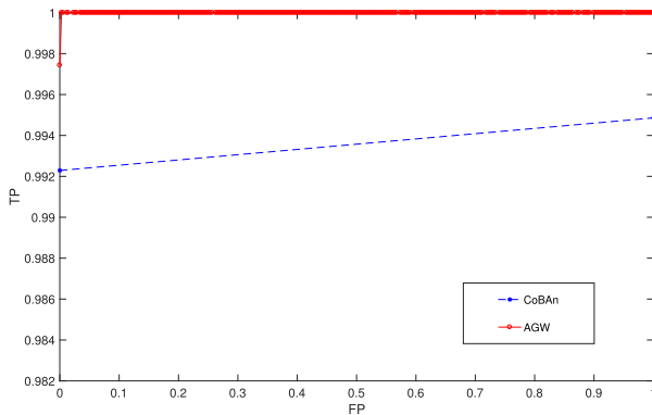
FIGURE 6. The ROC curves of CoBAn and AGW.
