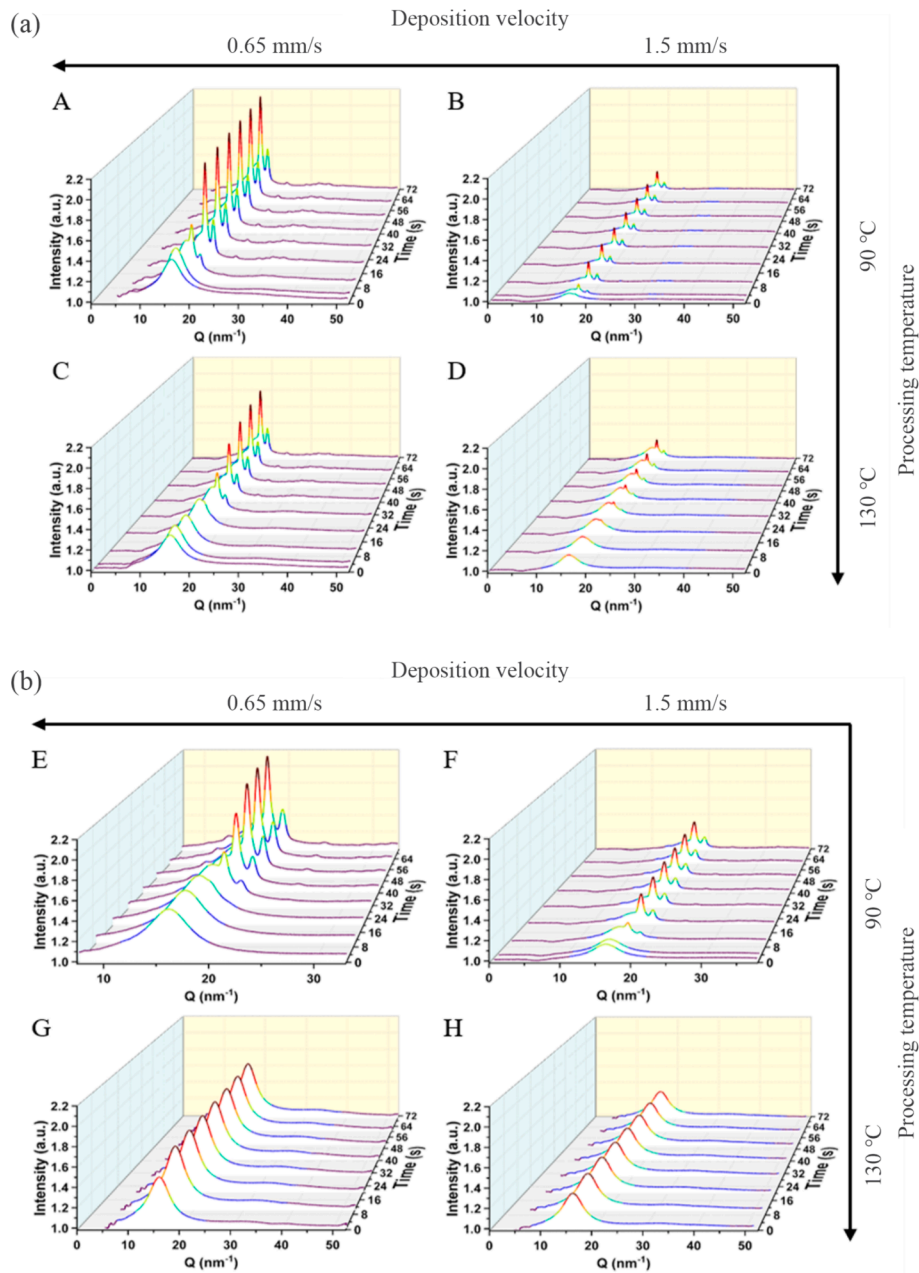
Fig. 3. In situ time-resolved XRD results of the (a) initial layer deposition (filaments printed on the stainless-steel platform), and (b) following layer deposition (filaments printed on the PCL structure surface) as a function of processing temperature and deposition velocity.
