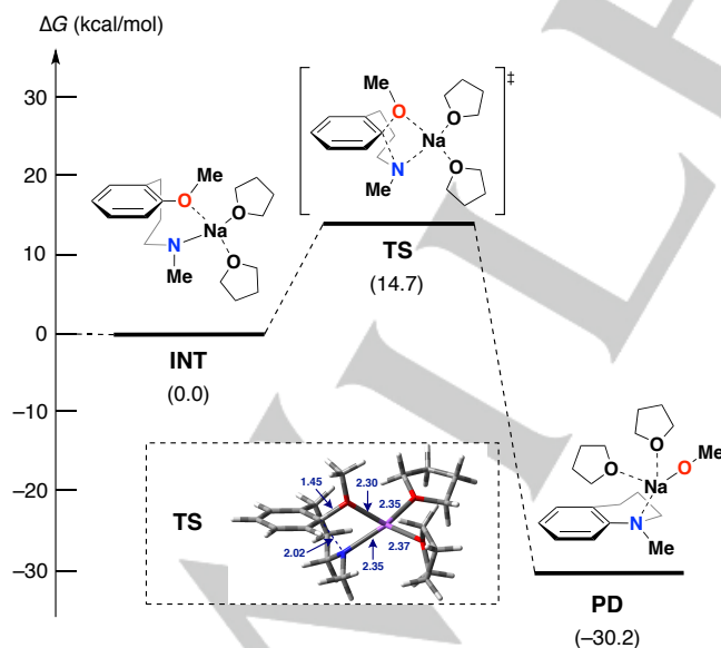
Figure 1. Reaction pathways of the nucleophilic amination with methoxy arenes. Energy changes and bond lengths at the B3LYP/6-31+G* level of theory (SCRF (pcm, solvent = THF)) are shown in kcal/mol and Å, respectively.
