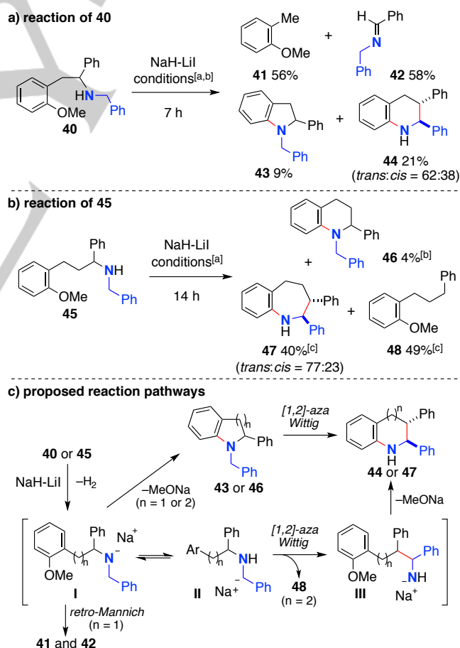
Scheme 5. Retro-Mannich reaction and skeletal rearrangement. [a] The reactions were conducted using 0.5 mmol of amines with NaH (3 equiv) and Lil (2 equiv) in THF (0.1 M) at 90 °C. [b] 1 H NMR yields. [c] Isolated yields.
