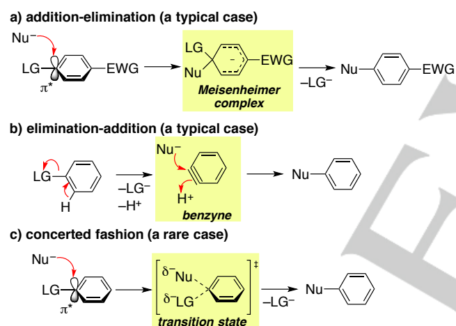
Scheme 1. Nucleophilic aromatic substitution reactions. Nu = nucleophile; EWG = electron withdrawing group; LG = leaving group
