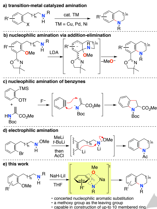
Scheme 2. Synthesis of benzannulated saturated nitrogen-heterocycles
