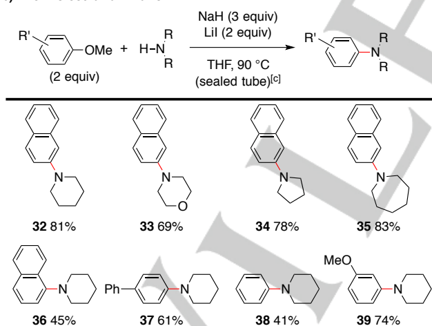
Scheme 4. Substrate scope. [a] The intramolecular reactions were conducted using 0.3–0.5 mmol of amines in THF (0.1 M) for 4–47 h and isolated yields of heterocycles were noted above unless otherwise stated. [b] NaH (6 equiv) and Lil (4 equiv) were used. PMB = para -methoxybenzyl. [c] The intermolecular reactions were conducted using amines (0.5 mmol) and methoxy arenes (1 mmol) in THF (1 M) for 40 h and isolated yields of aminated arenes were noted above.
