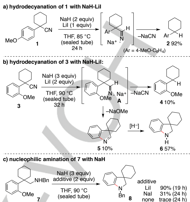
Scheme 3. Reactions with the NaH-iodide composite. [a] The reactions were conducted using 0.3–0.5 mmol of substrates in THF (0.1 M) and isolated yields of products were noted above. Bn = benzyl.
