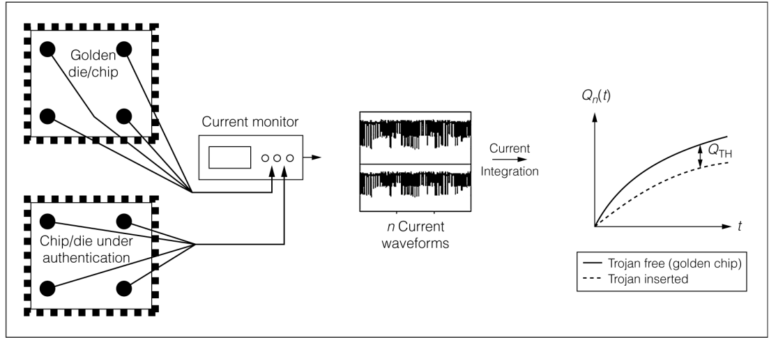
Figure 2.4: Power-based side-channel analysis [5].
