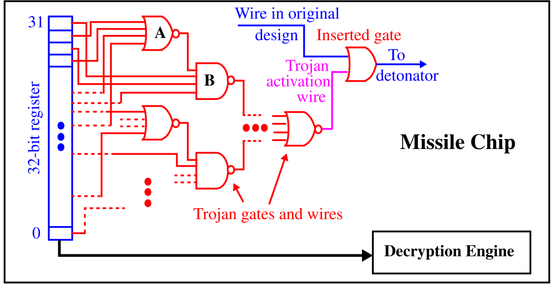
Figure 2.1: An example of hardware Trojan [2].
