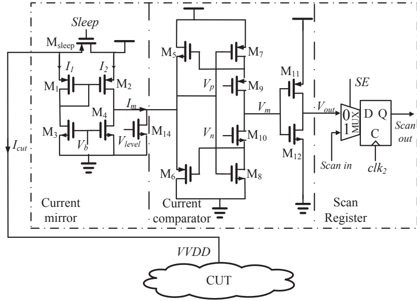
Figure 3.6: Schematic of the proposed current sensing to path delay monitoring circuit.
