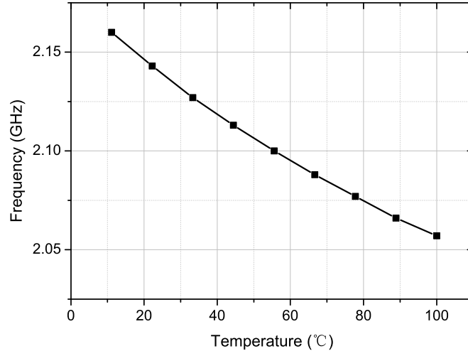
Figure 4.1: Change in oscillation frequency with temperature for an RO.
