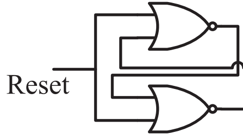
Figure 2.9: The logical structure of the latch PUF cell [9].
