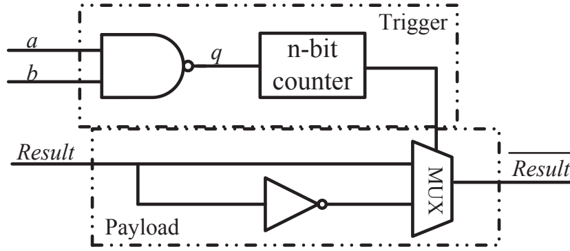
Figure 3.12: Counter-based Trojan circuit architecture [11].
