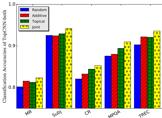
Fig. 8. Effects of different topics embeddings learning schemes on the whole five datasets. Here, we focus on TopCNN word&sen model with different kinds of input topics embeddings, while other parameters are kept the same. Different colors correspond to different topic embedding learning schemes. Random, additive, topical and joint represent topics embeddings generated from random model, additive model, topical neural model and joint neural model respectively.
