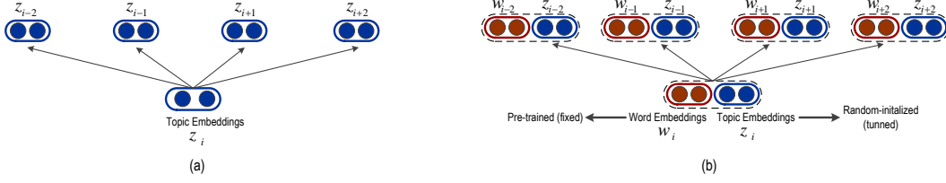
Fig. 5. Two neural network architectures (Skip-gram based) for topic embeddings learning: (a) Topical Neural Model; (b) Joint Neural Model.
