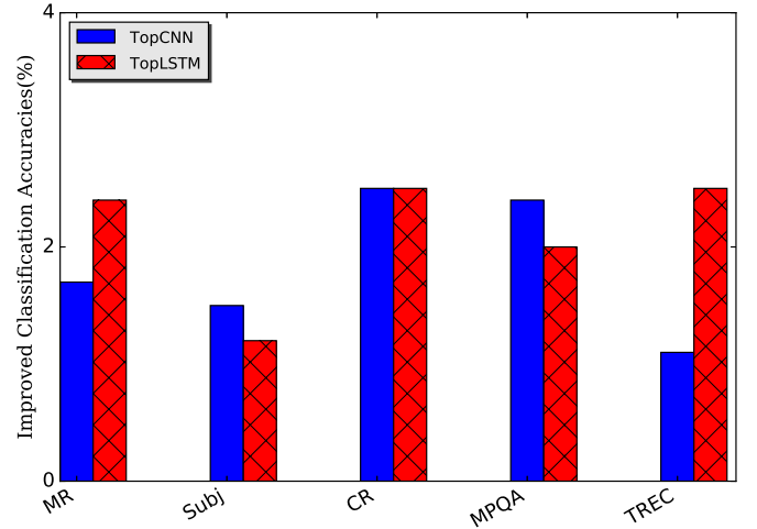
Fig. 6. Performances gains achieved by our proposed TopCNN and TopLSTMs models compared to CNN and LSTM, respectively
