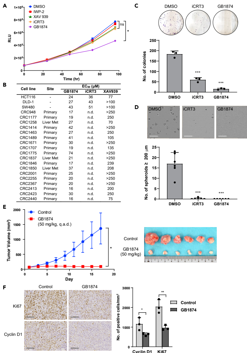
Figure 4. GB1874 inhibited growth of Wnt-driven cells in vitro and in vivo
