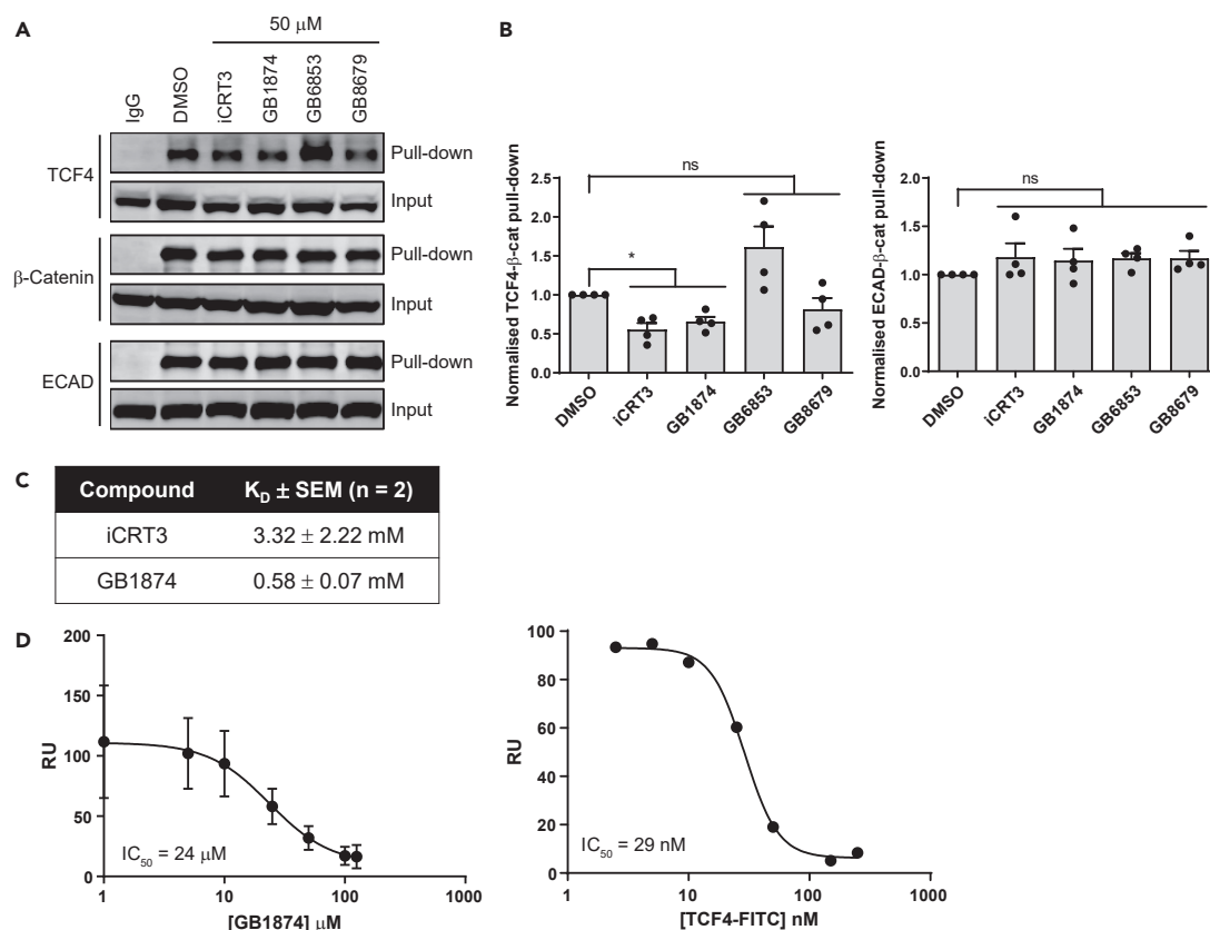
Figure 3. GB1874 inhibits Wnt signaling by disrupting \beta -cat-TCF4 interaction
