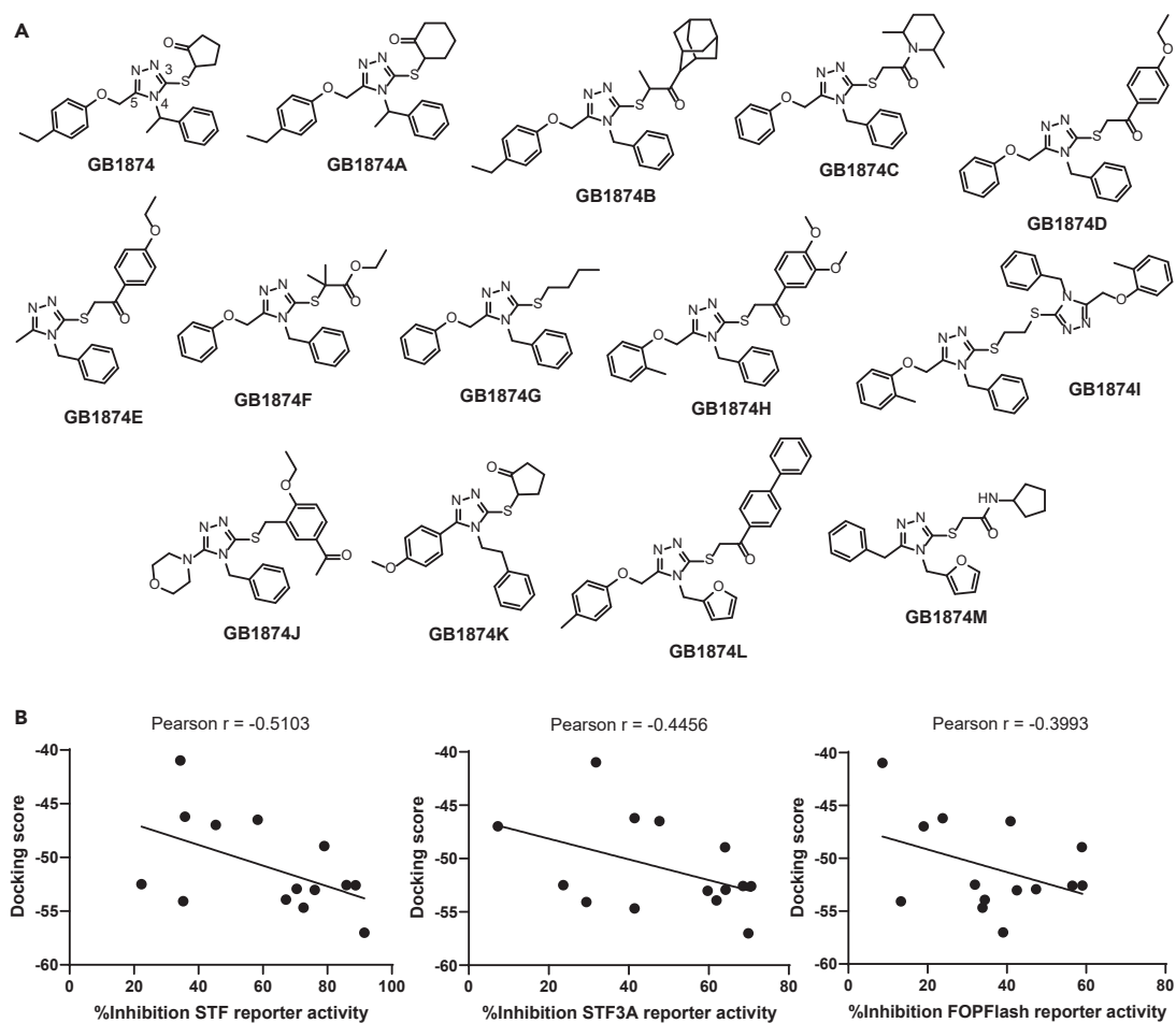
Figure 5. Structural analogs of GB1874 were also potent inhibitors of Wnt signaling
