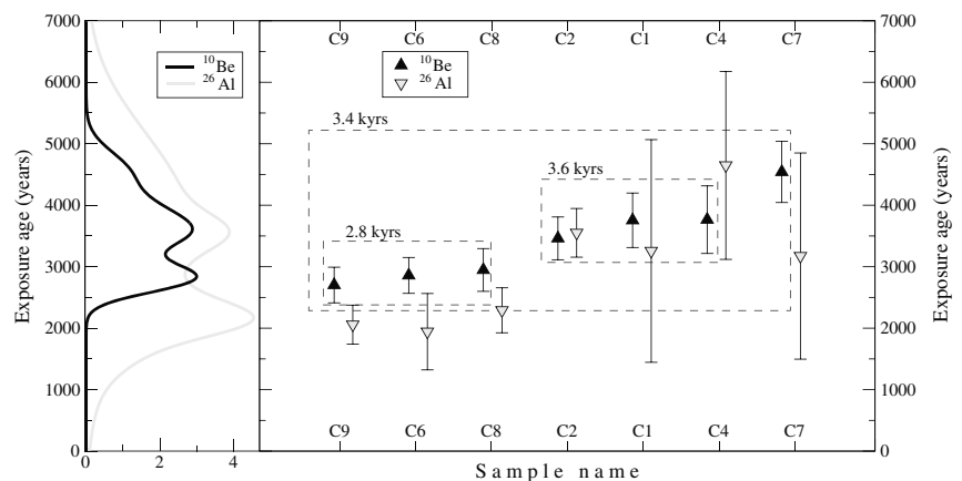
Figure 14. Cosmogenic ^{10}\text{Be} and ^{26}\text{Al} exposure ages of 7 (out of 11) sandstone cobbles collected on top surface of hanging wall terrace Th6 on Sir Khola east bank, 30 m above river. The boxes delineate the clusters of ages discussed in the text section 6.1.5. (left) Stacked probability distributions of ^{10}\text{Be} and ^{26}\text{Al} ages, with corresponding uncertainties imply \sim 3 ka final abandonment age.
