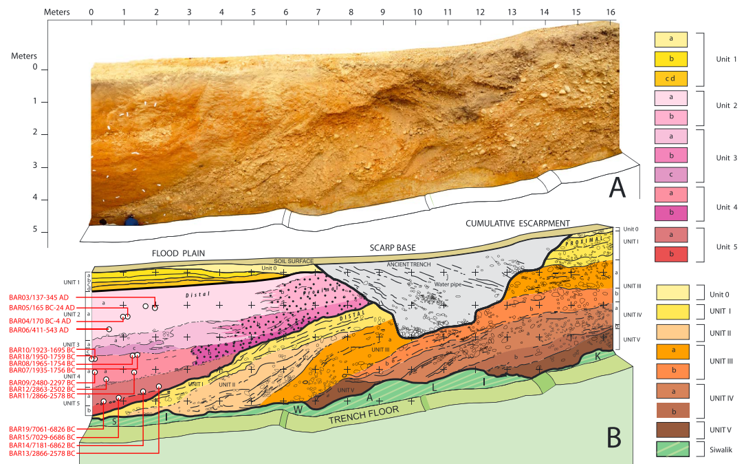
Figure 19. Thapatol trench, across main scarp in Figure 18c. (a) Photomosaic of 16 m long, south part of trench western wall. No fault was found down to \approx 5 m, implying flexural-folding origin of scarp. Distal, red-brown, sandy/clayey layers with occasional thin pebbly beds at base of scarp onlap coarse, poorly sorted, fluvial fanglomerates dipping \approx 20^\circ SW on top of scarp. The gravel layers in turn abrade deeper Siwalik beds. (b) Structural and stratigraphic log of wall shown in Figure 19a. Note area (in grey) completely disrupted by digging of older, smaller trench. Calibrated, calendric ^{14}\text{C} ages (red) of detrital charcoals within onlapping units of wash deposits at foot of scarp are positioned with white circles. See methodology appendix for calibration details.
