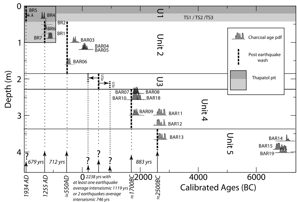
Figure 20. Synthetic plot, as a function of depth, of calibrated calendric ^{14}\text{C} ages of detrital charcoals collected within red sand/clay wash deposit units at base of flexural fold scarp, in both (top) Thapatol pit (location on Figure 18) and (bottom) trench (Figure 19). Successive, discrete episodes of wash influx are interpreted to postdate seismic growth increments of flexural fold scarp. Bold, dashed vertical lines mark inferred ages of corresponding events (see discussion in text).
