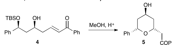
Scheme 2. Acid catalysed formation of the 2,6- cis isomer in a synthesis of diospongin A.
