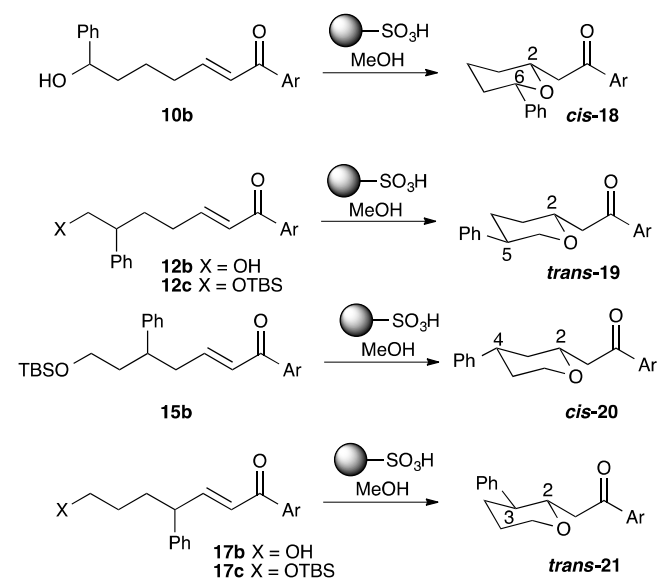
Scheme 9. Acid catalyzed cyclisation reactions. All reactions were carried out at room temperature. Ar = p -BrC 6 H 4 .
