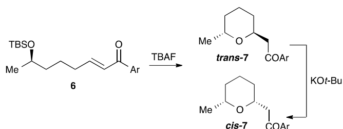
Scheme 4. Oxa-Michael addition in the synthesis of curvulone B with a non-coordinating counter ion.
