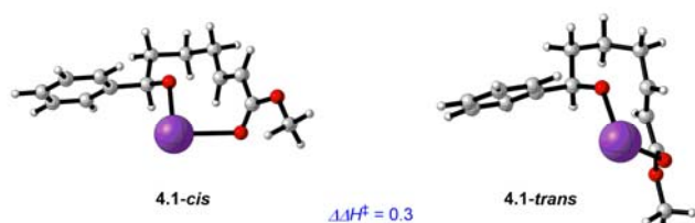
Figure 4. 2,6- cis and 2,6- trans transition states in the chelation model with potassium and the enthalpy difference (in kcal/mol) with respect to one other.
