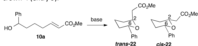
Scheme 11. Base catalyzed formation of the 2,6-disubstitution pattern. 20
