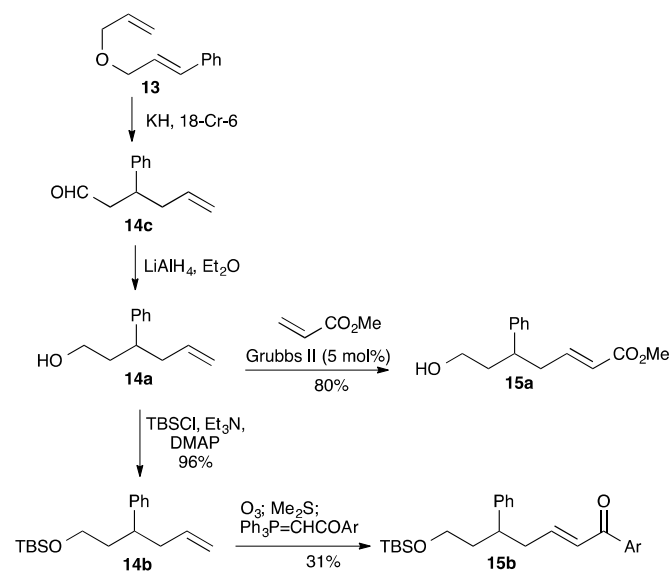
Scheme 7. Synthesis of substrates leading to 2,4-disubstitution. Ar = p -BrC 6 H 4 .
