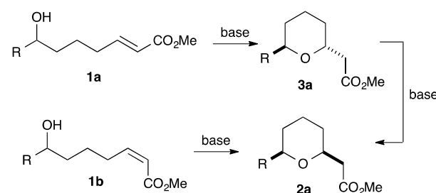
Scheme 3. Base catalysed formation of either isomer
