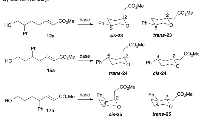
Scheme 12. Base catalysed formation with the other disubstitution patterns. 20
