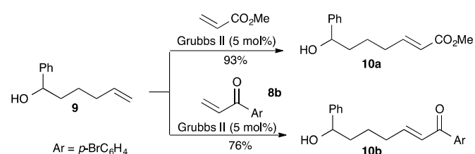
Scheme 5. Synthesis of substrates leading to 2,6-disubstitution. Ar = p -BrC 6 H 4 .
