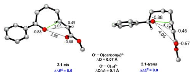
Figure 5. Electrostatic interactions in the TS of the base catalysed reaction. Distances in Å.
