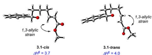
Figure 3. Transition states with s -trans Michael acceptors having 1,3-allylic strain and their relative enthalpies (in kcal/mol) with respect to SM-anion.
