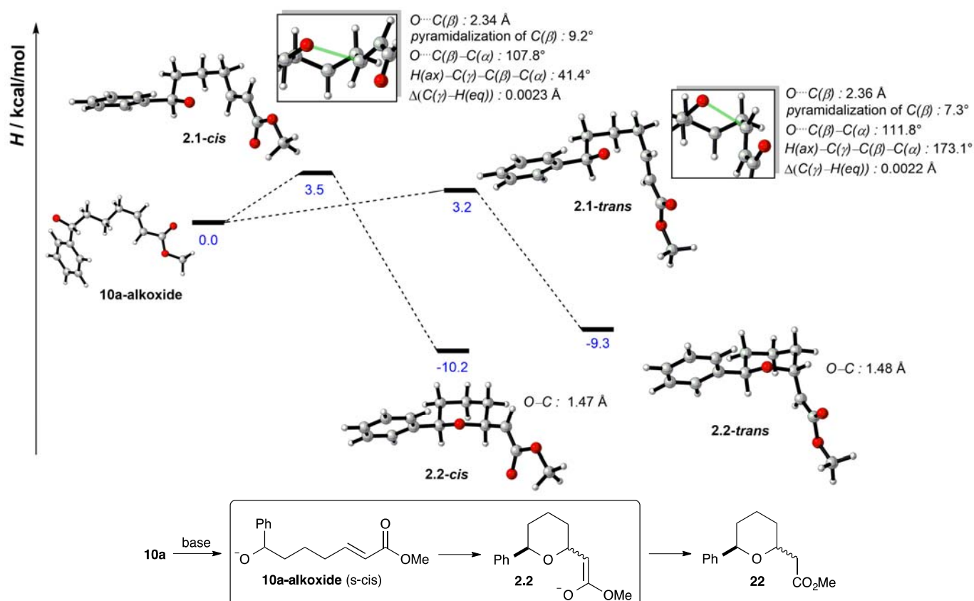
Figure 2. Enthalpy profile for the base-catalysed cyclisation. Gibbs Free Energy values are not shown as they predict a stereochemical outcome opposite to that observed (see S.I. for more details).
