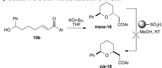
Scheme 10. Non-equilibration under acidic conditions. Ar = p -BrC 6 H 4 .
