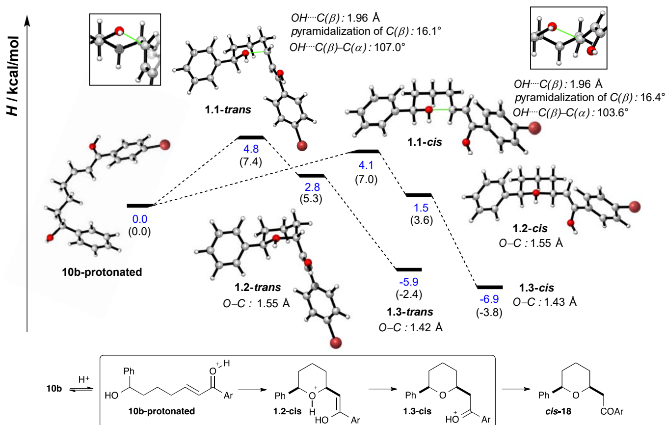
Figure 1. Enthalpy profile for the acid-catalysed oxa -Michael cyclisation. Gibbs Free Energies are shown in parentheses.
