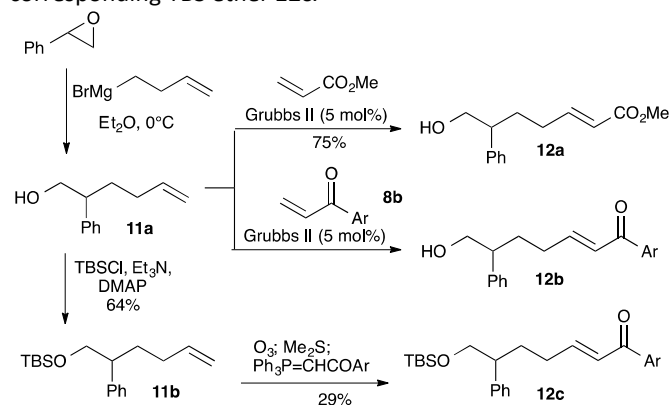
Scheme 6. Synthesis of substrates leading to 2,5-disubstitution. Ar = p -BrC 6 H 4 .
