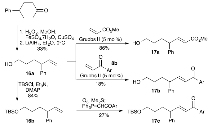
Scheme 8. Synthesis of substrates leading to 2,3-disubstitution. Ar = p -BrC 6 H 4 .
