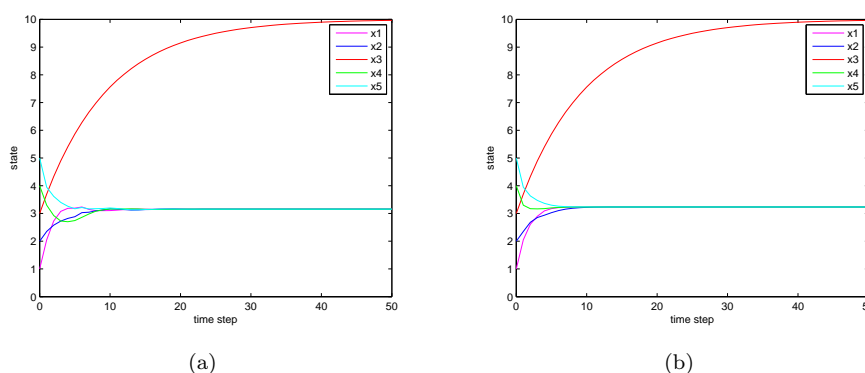
Figure 2. State trajectories of all agents with and without a transmission delay.
