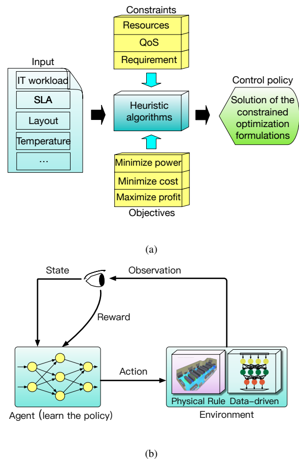
Fig. 3. The workflows of a) existing approaches and b) DRL-based approach. (SLA: Service Level Agreement; QoS: Quality of Service.) The existing approaches assume some static models for the system but often cannot solve the extremely complicated constrained optimization problems due to the complexity of the models. Meanwhile, Our proposed DRL-based approach iteratively interacts with the target system and automatically learns the optimal control policies without solving the complicated constrained optimization formulations explicitly.
